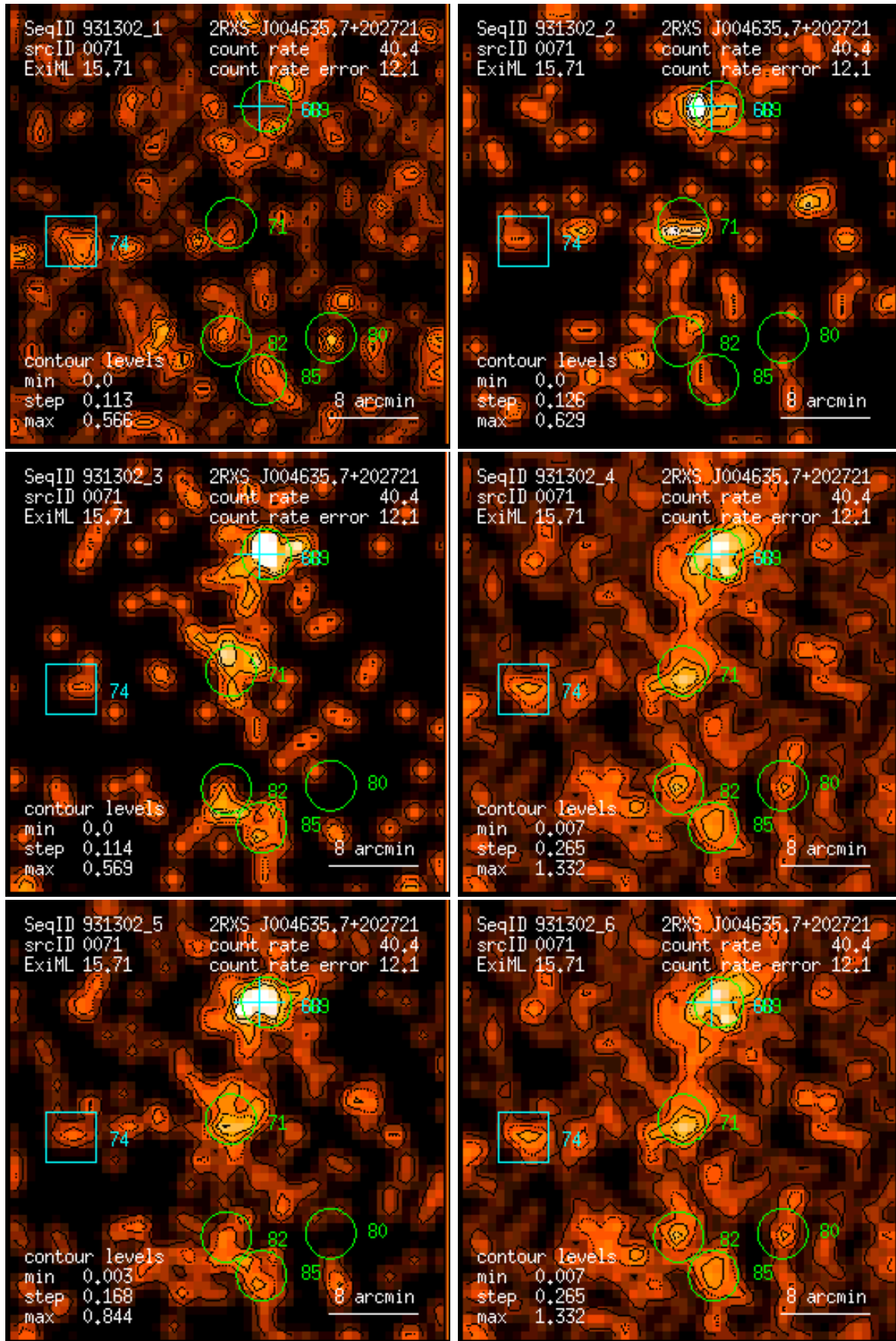
Figure 71: RASS 931302: detection 0071: band rate images, Gaussian filter: (1) PSPC channels 11 – 41, (2) 52 – 90, (3) 91 – 201, (4) 11 – 235, (5) 52 – 201, (6) 11 – 201. Broad band rates in counts/ks. Band rate contour levels in counts/ks/arcmin 2 .
