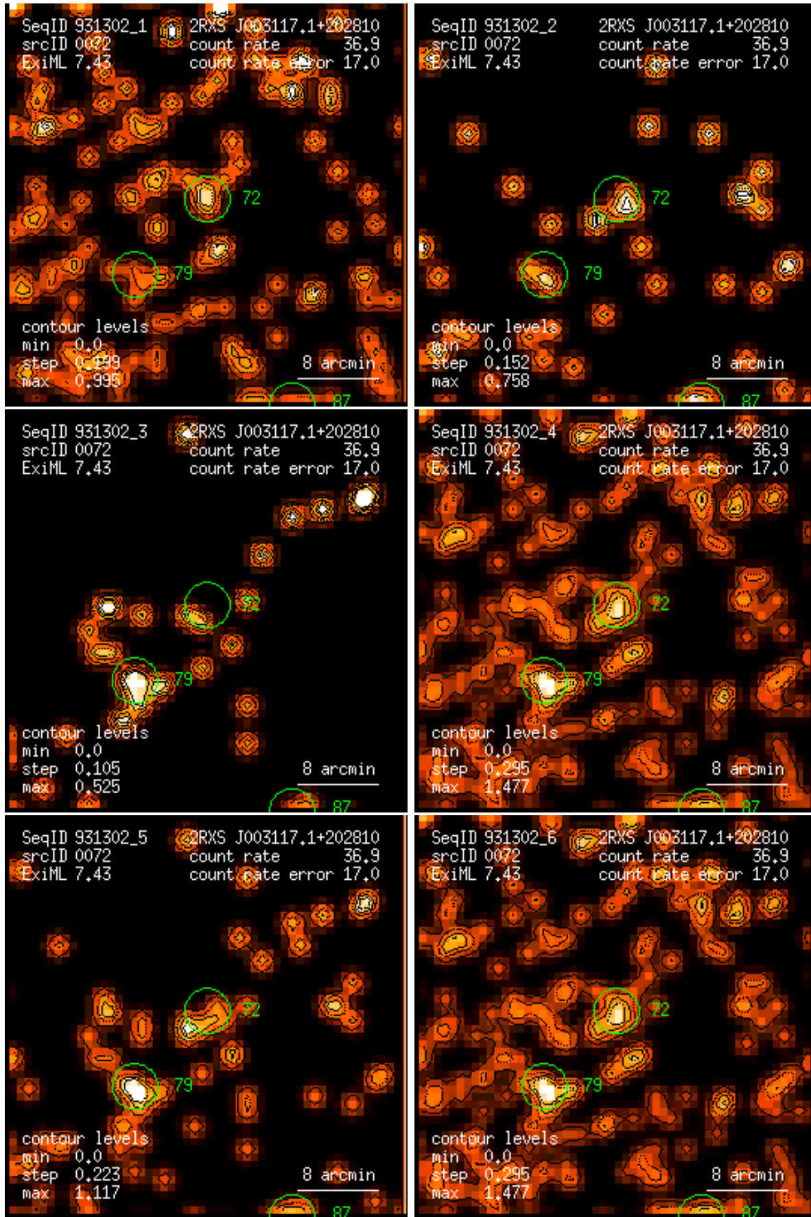
Figure 72: RASS 931302: detection 0072: band rate images, Gaussian filter: (1) PSPC channels 11 – 41, (2) 52 – 90, (3) 91 – 201, (4) 11 – 235, (5) 52 – 201, (6) 11 – 201. Broad band rates in counts/ks. Band rate contour levels in counts/ks/arcmin 2 .
