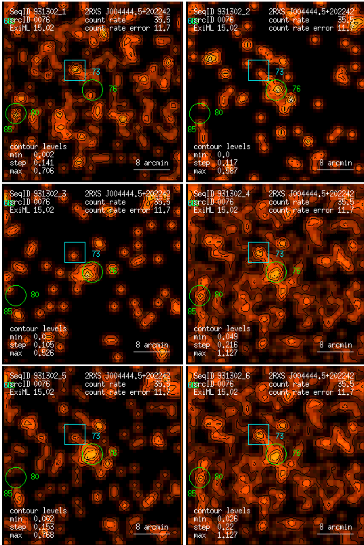
Figure 76: RASS 931302: detection 0076: band rate images, Gaussian filter: (1) PSPC channels 11 – 41, (2) 52 – 90, (3) 91 – 201, (4) 11 – 235, (5) 52 – 201, (6) 11 – 201. Broad band rates in counts/ks. Band rate contour levels in counts/ks/arcmin 2 .
