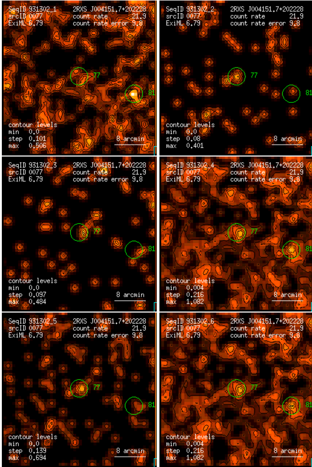
Figure 77: RASS 931302: detection 0077: band rate images, Gaussian filter: (1) PSPC channels 11 – 41, (2) 52 – 90, (3) 91 – 201, (4) 11 – 235, (5) 52 – 201, (6) 11 – 201. Broad band rates in counts/ks. Band rate contour levels in counts/ks/arcmin 2 .
