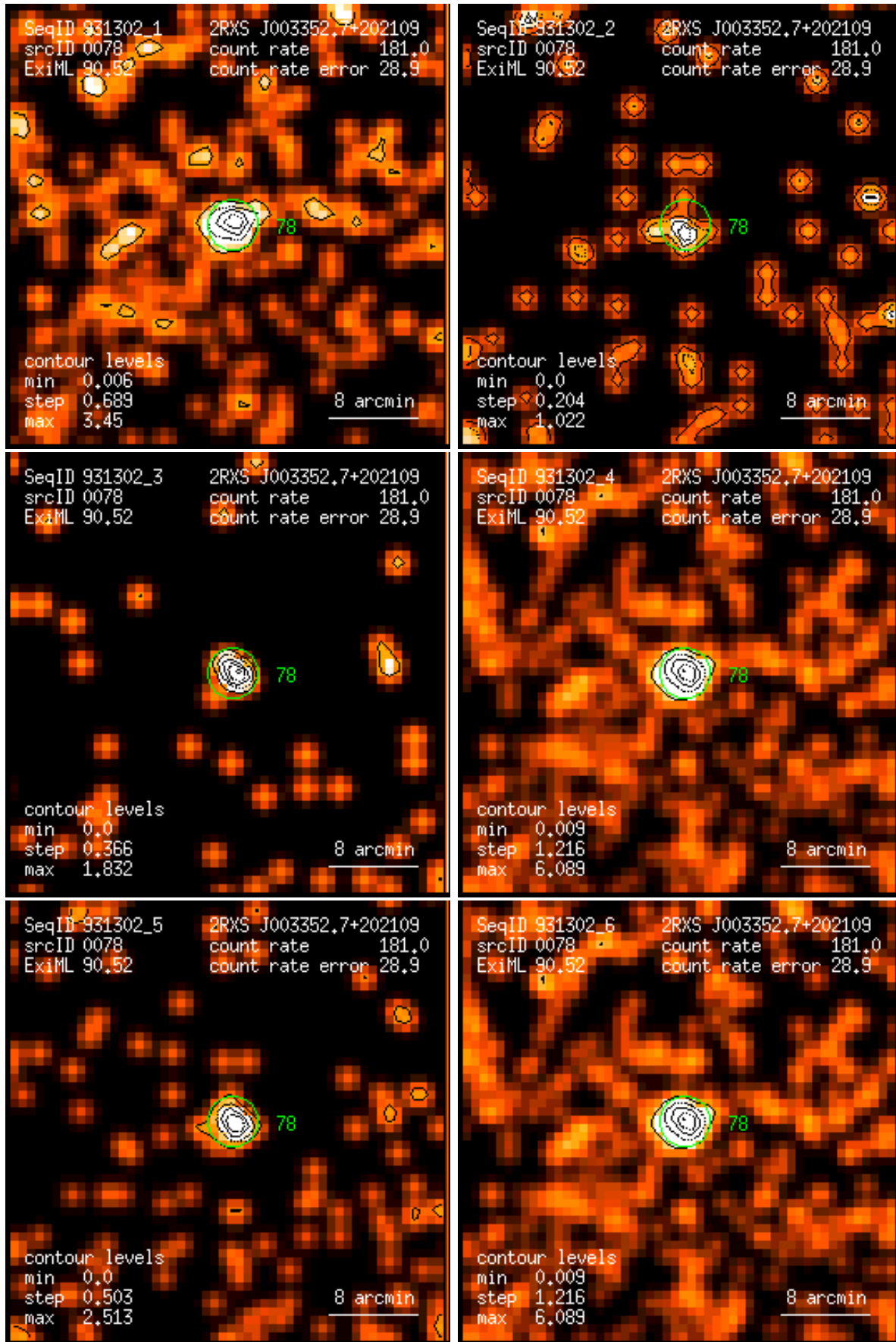
Figure 78: RASS 931302: detection 0078: band rate images, Gaussian filter: (1) PSPC channels 11 – 41, (2) 52 – 90, (3) 91 – 201, (4) 11 – 235, (5) 52 – 201, (6) 11 – 201. Broad band rates in counts/ks. Band rate contour levels in counts/ks/arcmin 2 .
