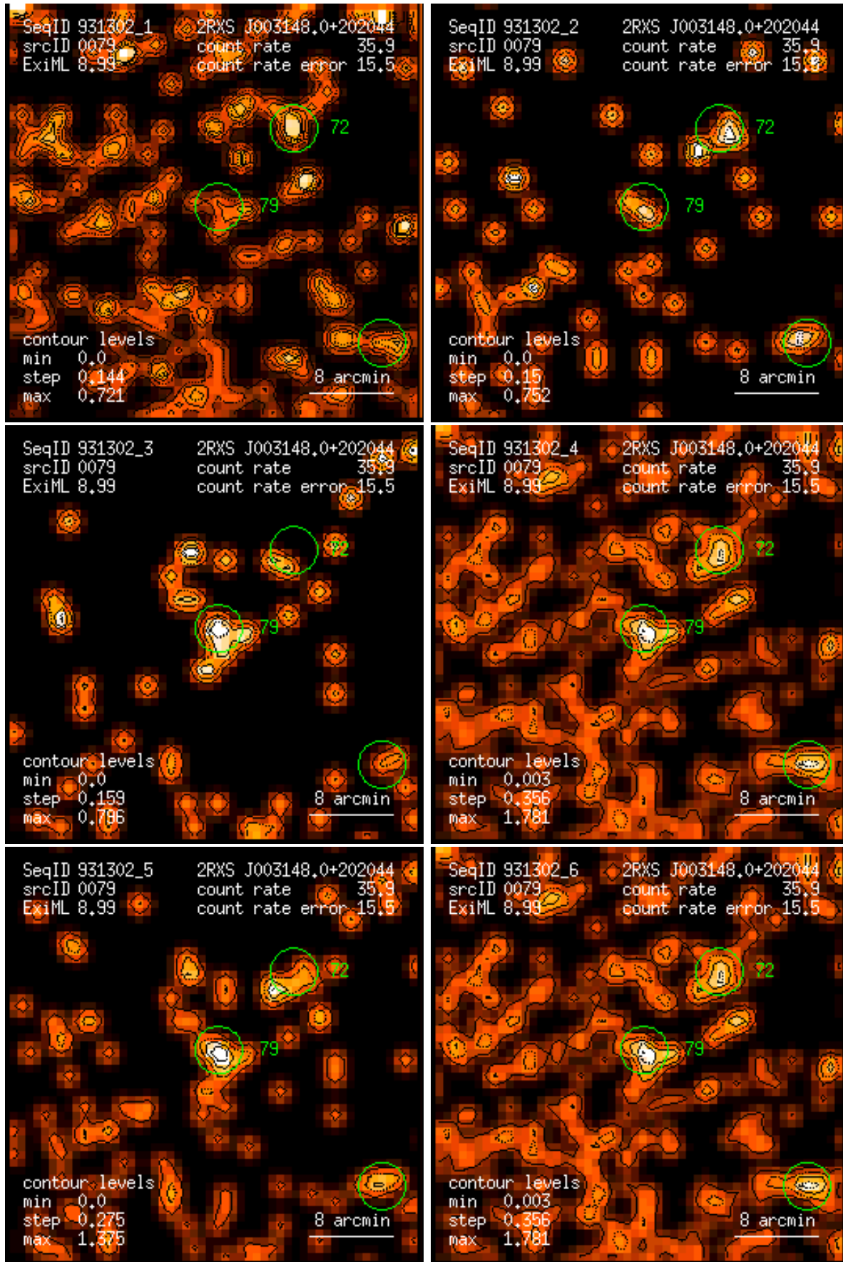
Figure 79: RASS 931302: detection 0079: band rate images, Gaussian filter: (1) PSPC channels 11 – 41, (2) 52 – 90, (3) 91 – 201, (4) 11 – 235, (5) 52 – 201, (6) 11 – 201. Broad band rates in counts/ks. Band rate contour levels in counts/ks/arcmin 2 .
