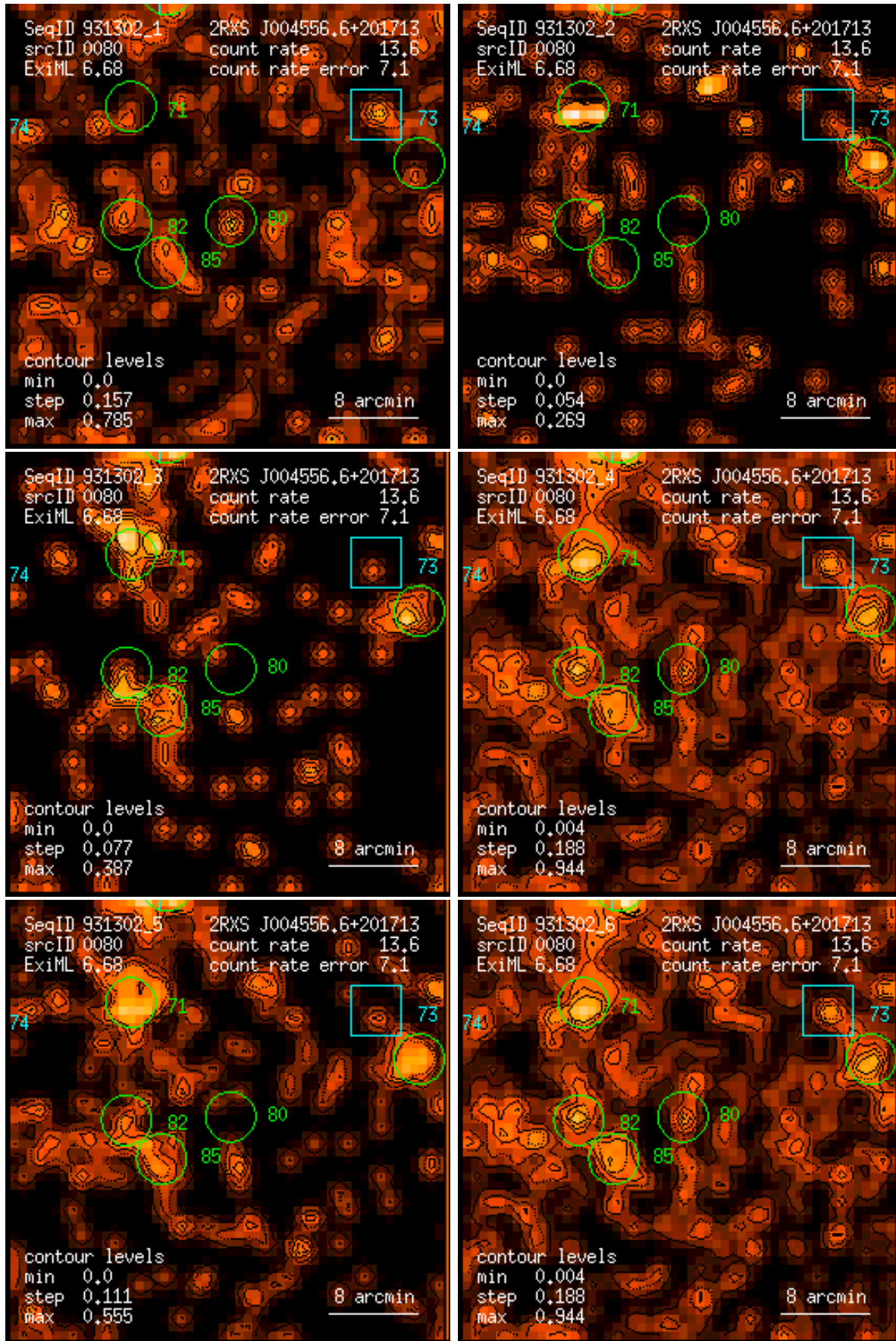
Figure 80: RASS 931302: detection 0080: band rate images, Gaussian filter: (1) PSPC channels 11 – 41, (2) 52 – 90, (3) 91 – 201, (4) 11 – 235, (5) 52 – 201, (6) 11 – 201. Broad band rates in counts/ks. Band rate contour levels in counts/ks/arcmin 2 .
