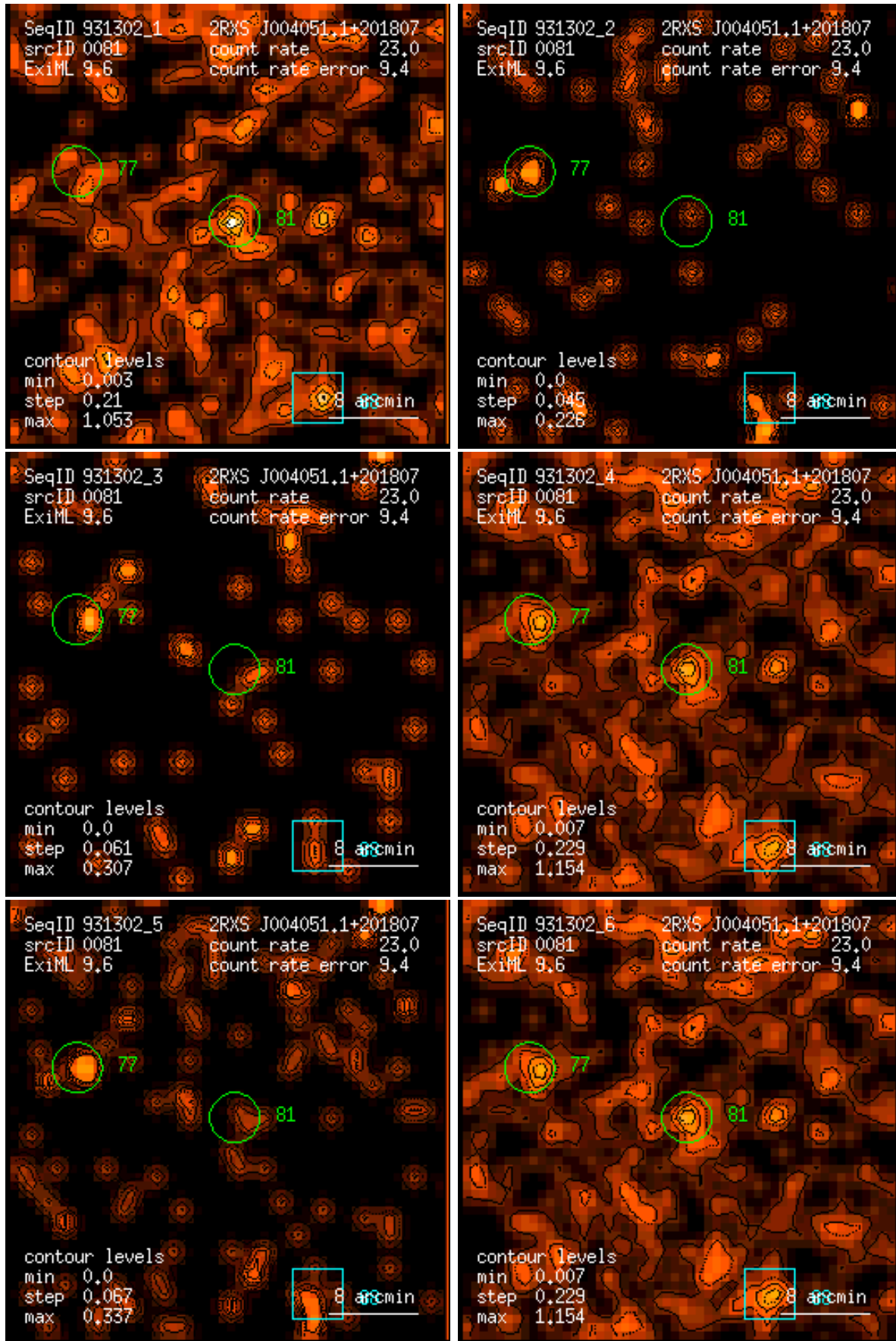
Figure 81: RASS 931302: detection 0081: band rate images, Gaussian filter: (1) PSPC channels 11 – 41, (2) 52 – 90, (3) 91 – 201, (4) 11 – 235, (5) 52 – 201, (6) 11 – 201. Broad band rates in counts/ks. Band rate contour levels in counts/ks/arcmin 2 .
