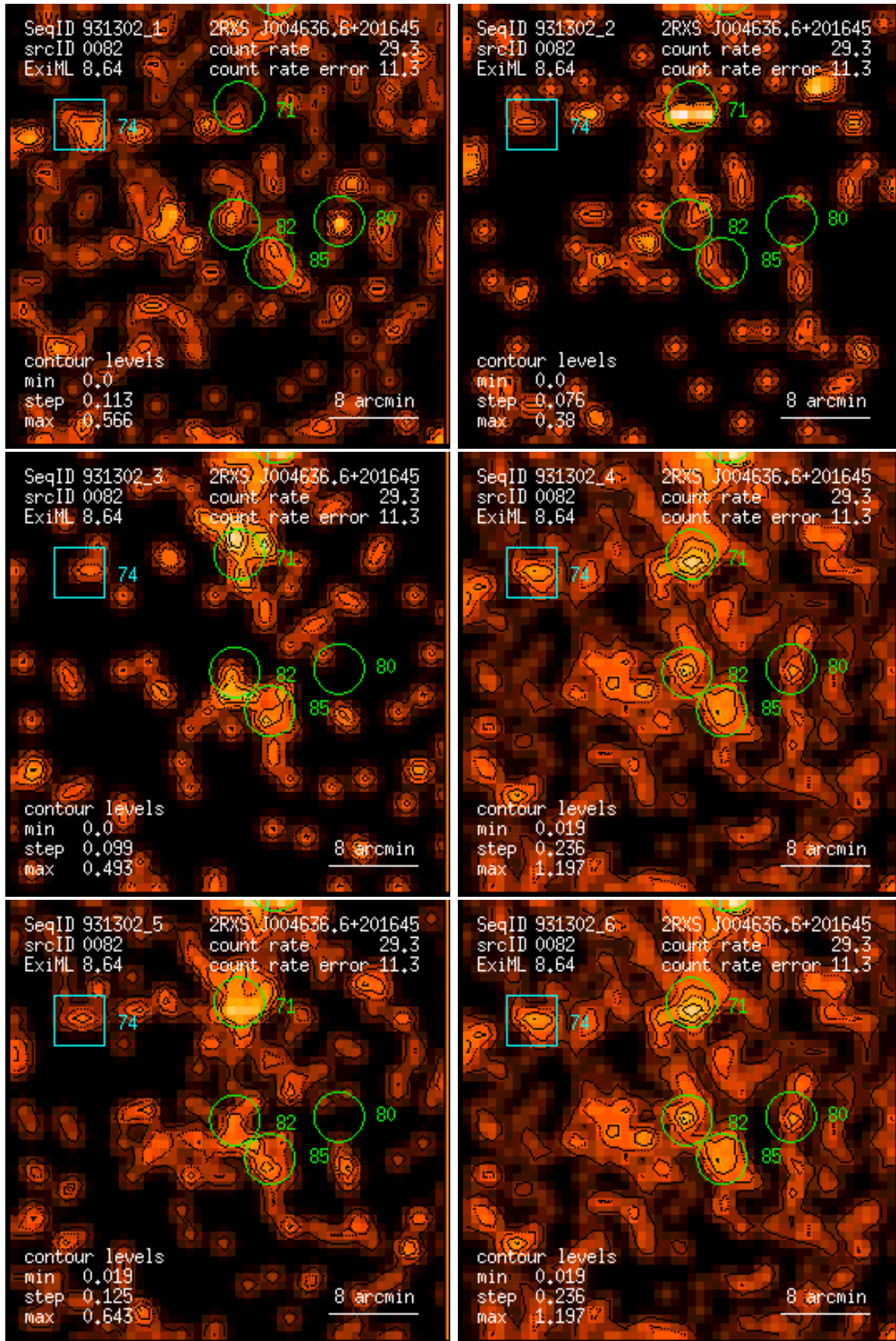
Figure 82: RASS 931302: detection 0082: band rate images, Gaussian filter: (1) PSPC channels 11 – 41, (2) 52 – 90, (3) 91 – 201, (4) 11 – 235, (5) 52 – 201, (6) 11 – 201. Broad band rates in counts/ks. Band rate contour levels in counts/ks/arcmin 2 .
