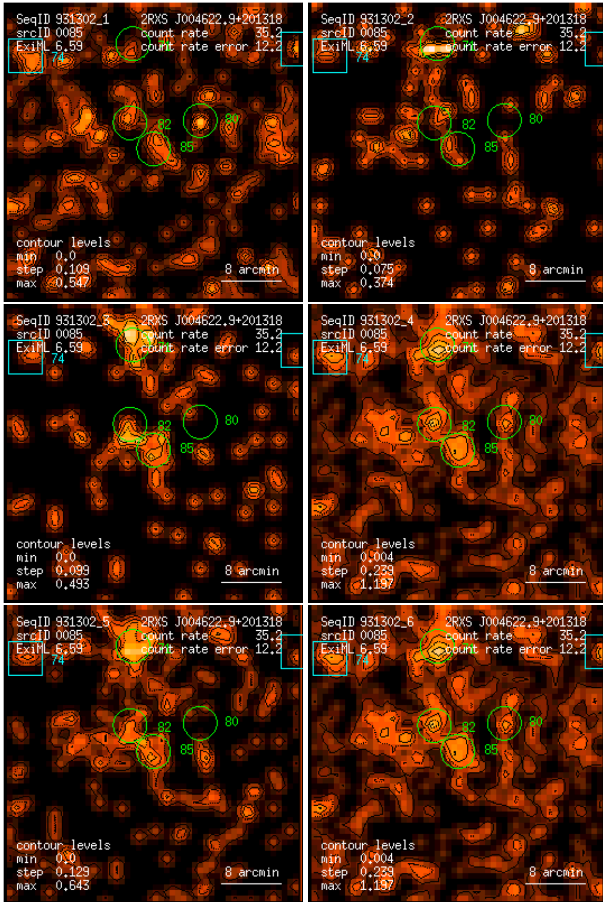
Figure 85: RASS 931302: detection 0085: band rate images, Gaussian filter: (1) PSPC channels 11 – 41, (2) 52 – 90, (3) 91 – 201, (4) 11 – 235, (5) 52 – 201, (6) 11 – 201. Broad band rates in counts/ks. Band rate contour levels in counts/ks/arcmin 2 .
