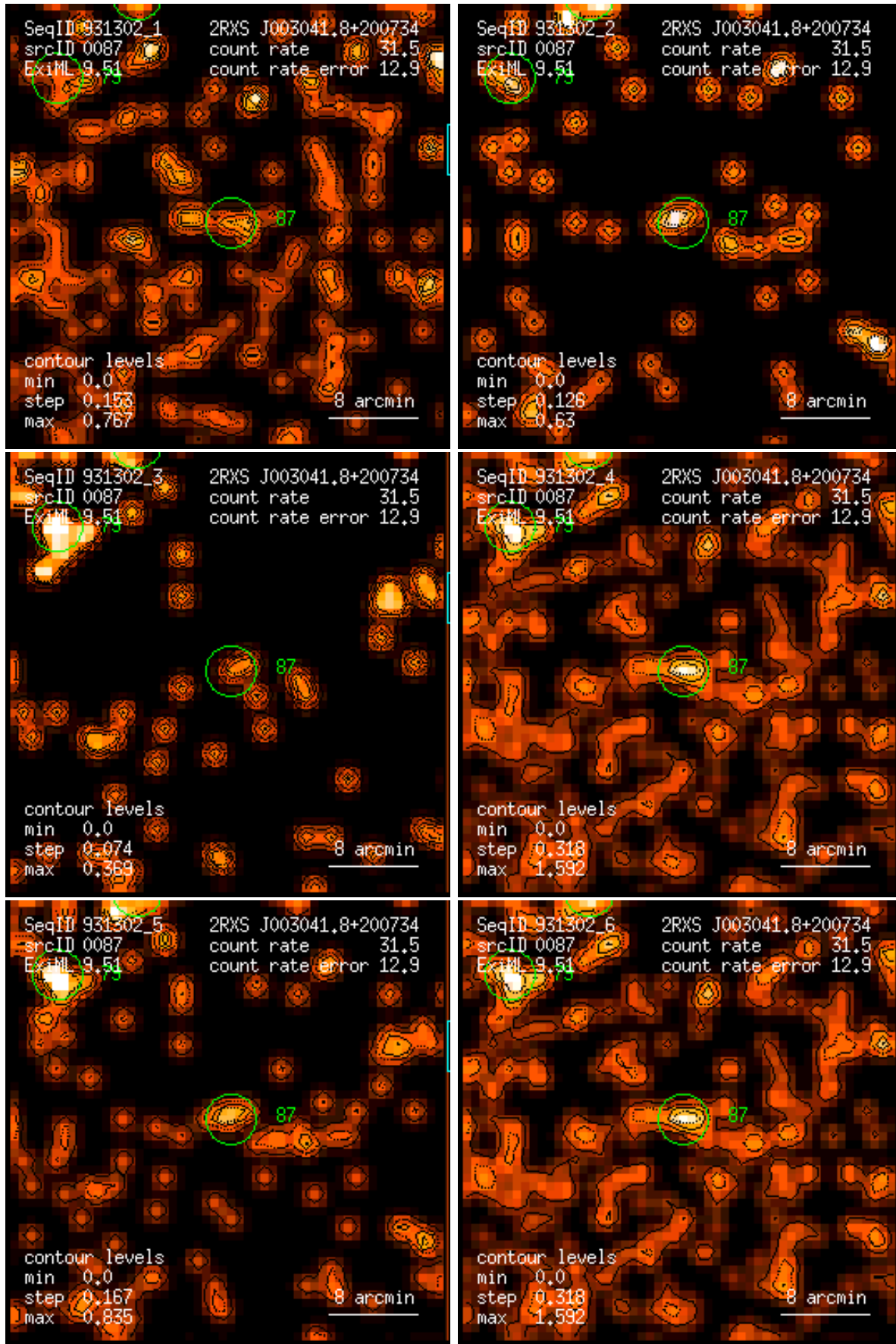
Figure 87: RASS 931302: detection 0087: band rate images, Gaussian filter: (1) PSPC channels 11 – 41, (2) 52 – 90, (3) 91 – 201, (4) 11 – 235, (5) 52 – 201, (6) 11 – 201. Broad band rates in counts/ks. Band rate contour levels in counts/ks/arcmin 2 .
