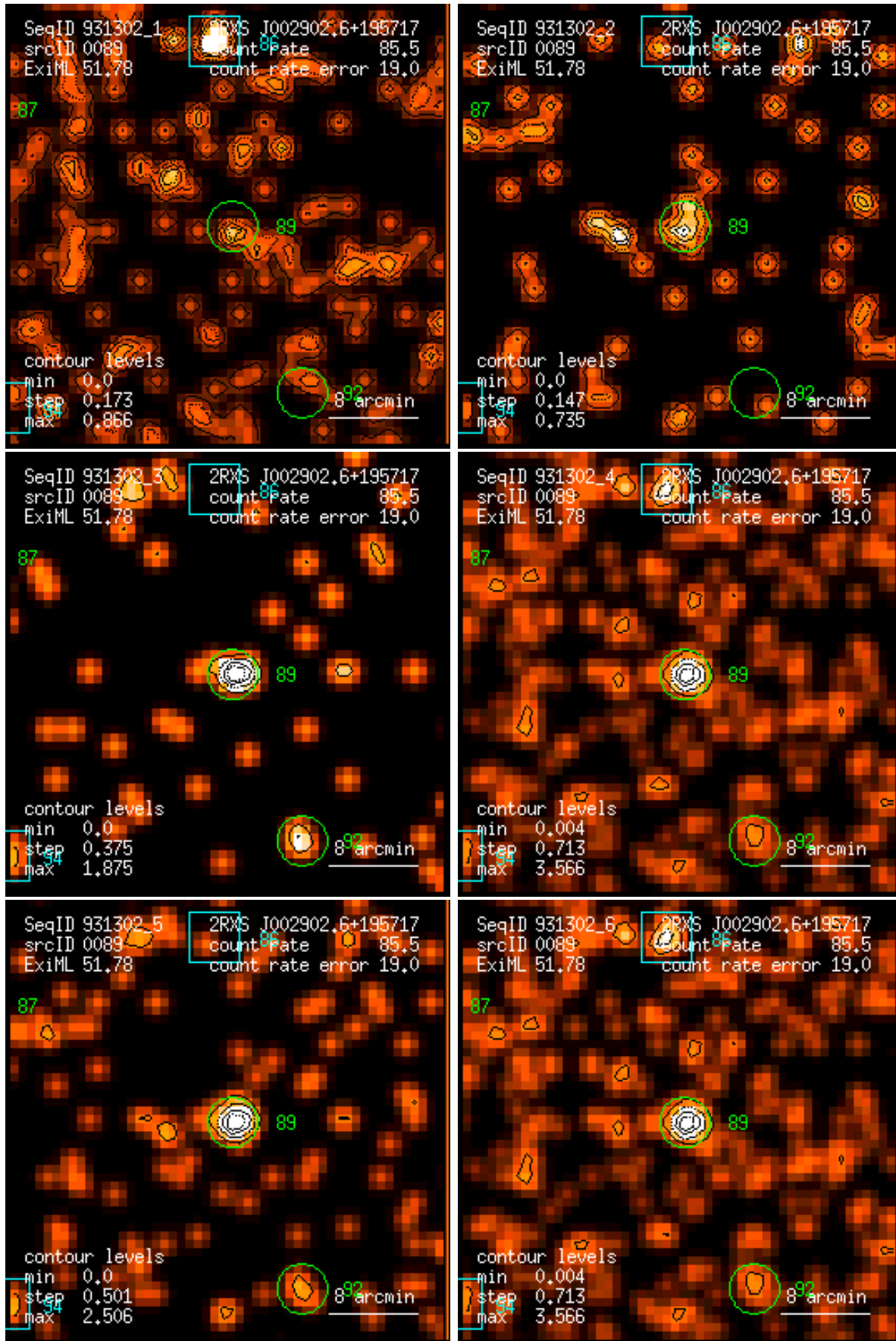
Figure 89: RASS 931302: detection 0089: band rate images, Gaussian filter: (1) PSPC channels 11 – 41, (2) 52 – 90, (3) 91 – 201, (4) 11 – 235, (5) 52 – 201, (6) 11 – 201. Broad band rates in counts/ks. Band rate contour levels in counts/ks/arcmin 2 .
