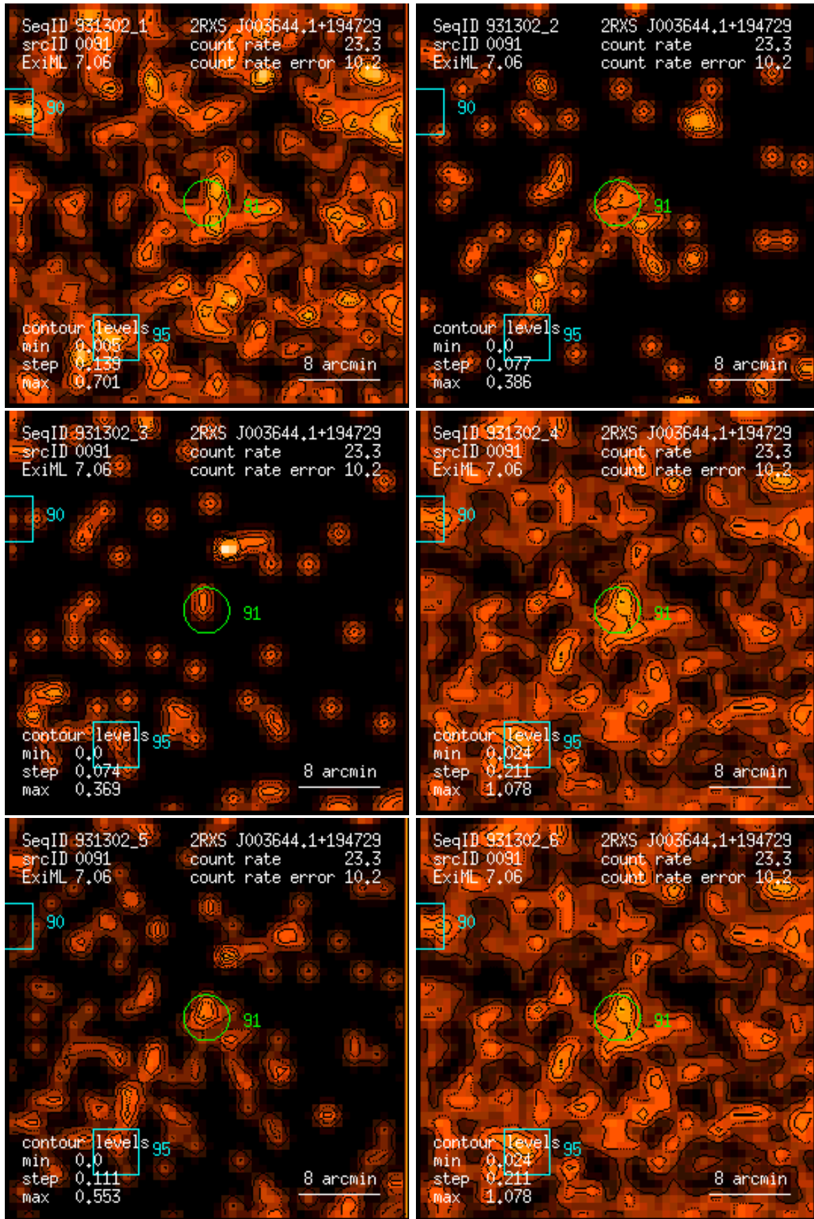
Figure 91: RASS 931302: detection 0091: band rate images, Gaussian filter: (1) PSPC channels 11 – 41, (2) 52 – 90, (3) 91 – 201, (4) 11 – 235, (5) 52 – 201, (6) 11 – 201. Broad band rates in counts/ks. Band rate contour levels in counts/ks/arcmin 2 .
