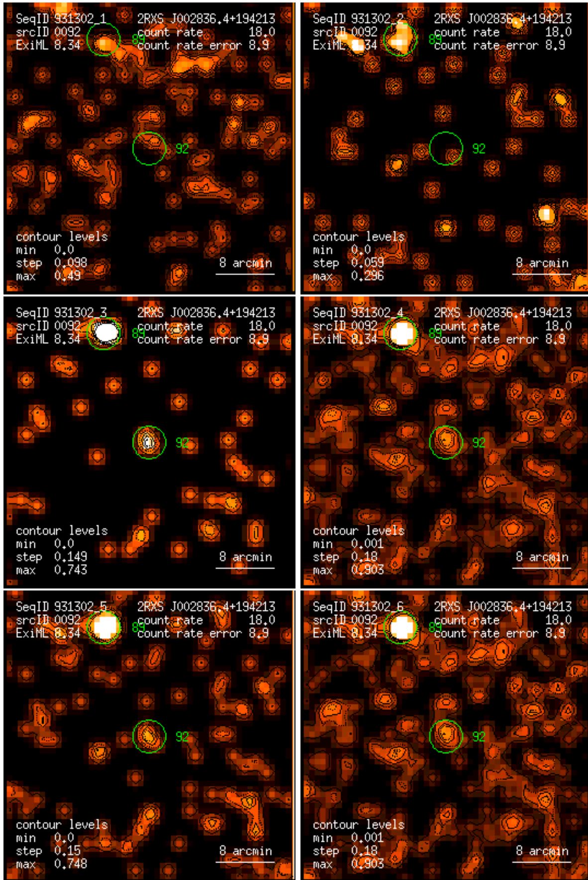
Figure 92: RASS 931302: detection 0092: band rate images, Gaussian filter: (1) PSPC channels 11 – 41, (2) 52 – 90, (3) 91 – 201, (4) 11 – 235, (5) 52 – 201, (6) 11 – 201. Broad band rates in counts/ks. Band rate contour levels in counts/ks/arcmin 2 .
