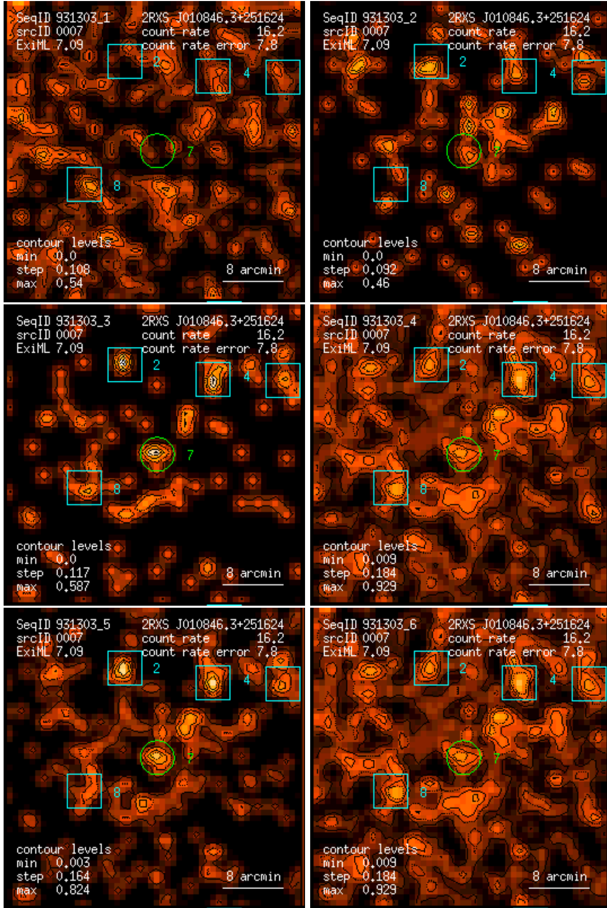
Figure 7: RASS 931303: detection 0007: band rate images, Gaussian filter: (1) PSPC channels 11 – 41, (2) 52 – 90, (3) 91 – 201, (4) 11 – 235, (5) 52 – 201, (6) 11 – 201. Broad band rates in counts/ks. Band rate contour levels in counts/ks/arcmin 2 .
