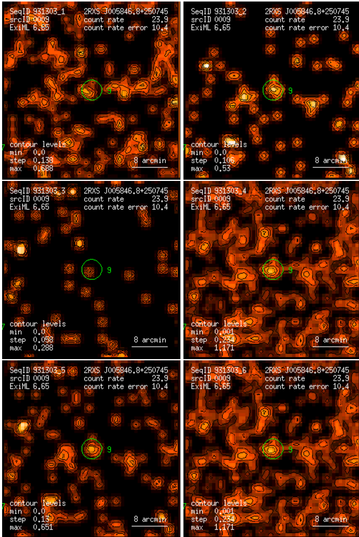
Figure 9: RASS 931303: detection 0009: band rate images, Gaussian filter: (1) PSPC channels 11 – 41, (2) 52 – 90, (3) 91 – 201, (4) 11 – 235, (5) 52 – 201, (6) 11 – 201. Broad band rates in counts/ks. Band rate contour levels in counts/ks/arcmin 2 .
