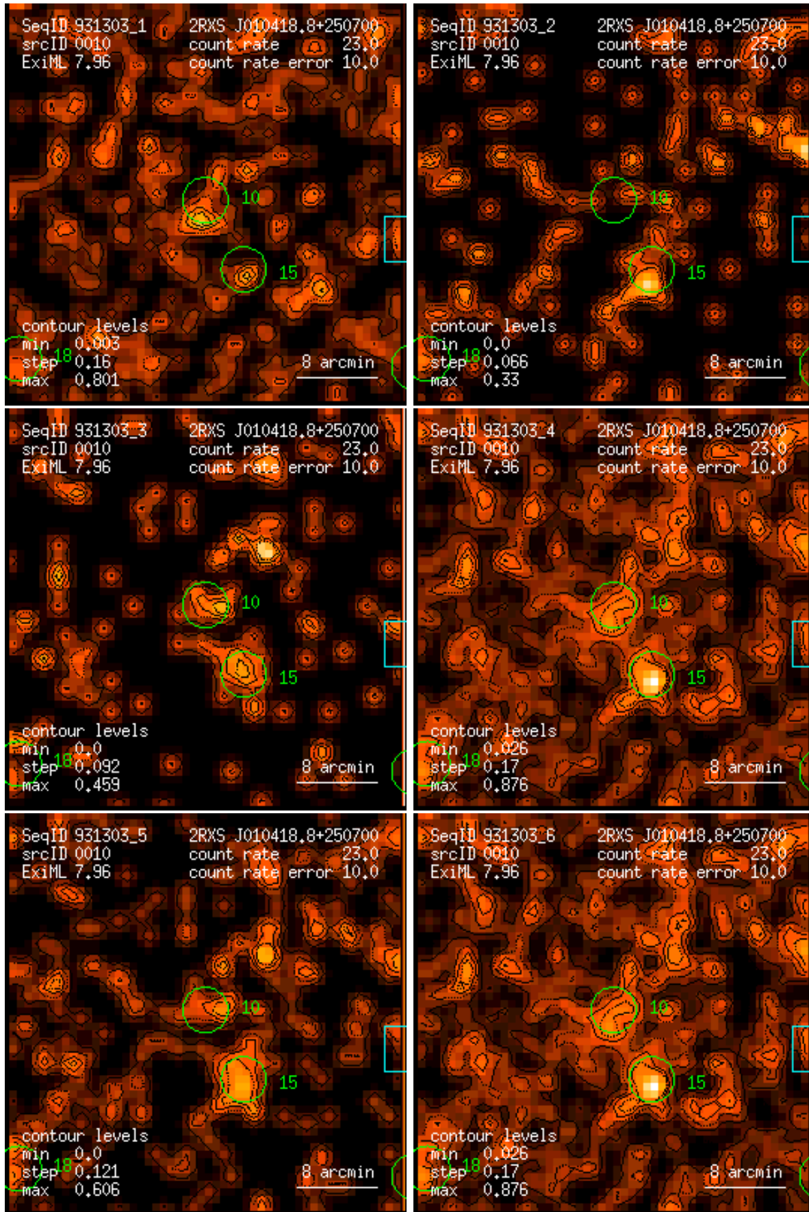
Figure 10: RASS 931303: detection 0010: band rate images, Gaussian filter: (1) PSPC channels 11 – 41, (2) 52 – 90, (3) 91 – 201, (4) 11 – 235, (5) 52 – 201, (6) 11 – 201. Broad band rates in counts/ks. Band rate contour levels in counts/ks/arcmin 2 .
