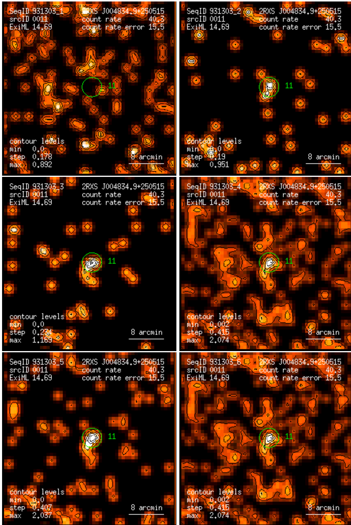
Figure 11: RASS 931303: detection 0011: band rate images, Gaussian filter: (1) PSPC channels 11 – 41, (2) 52 – 90, (3) 91 – 201, (4) 11 – 235, (5) 52 – 201, (6) 11 – 201. Broad band rates in counts/ks. Band rate contour levels in counts/ks/arcmin 2 .
