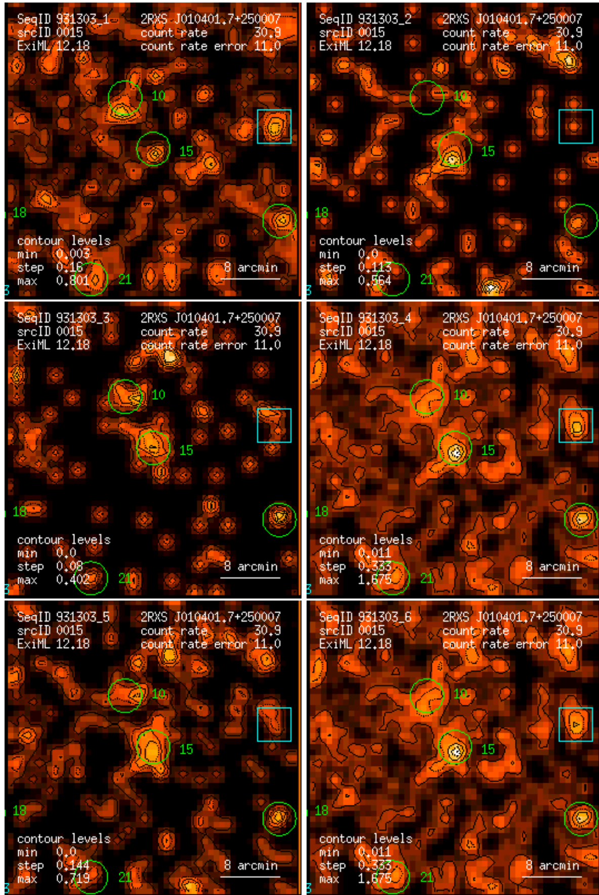
Figure 15: RASS 931303: detection 0015: band rate images, Gaussian filter: (1) PSPC channels 11 – 41, (2) 52 – 90, (3) 91 – 201, (4) 11 – 235, (5) 52 – 201, (6) 11 – 201. Broad band rates in counts/ks. Band rate contour levels in counts/ks/arcmin 2 .
