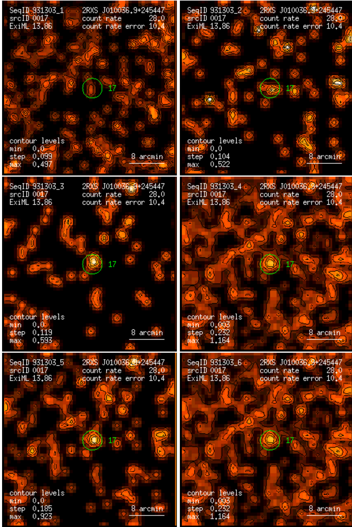
Figure 17: RASS 931303: detection 0017: band rate images, Gaussian filter: (1) PSPC channels 11 – 41, (2) 52 – 90, (3) 91 – 201, (4) 11 – 235, (5) 52 – 201, (6) 11 – 201. Broad band rates in counts/ks. Band rate contour levels in counts/ks/arcmin 2 .
