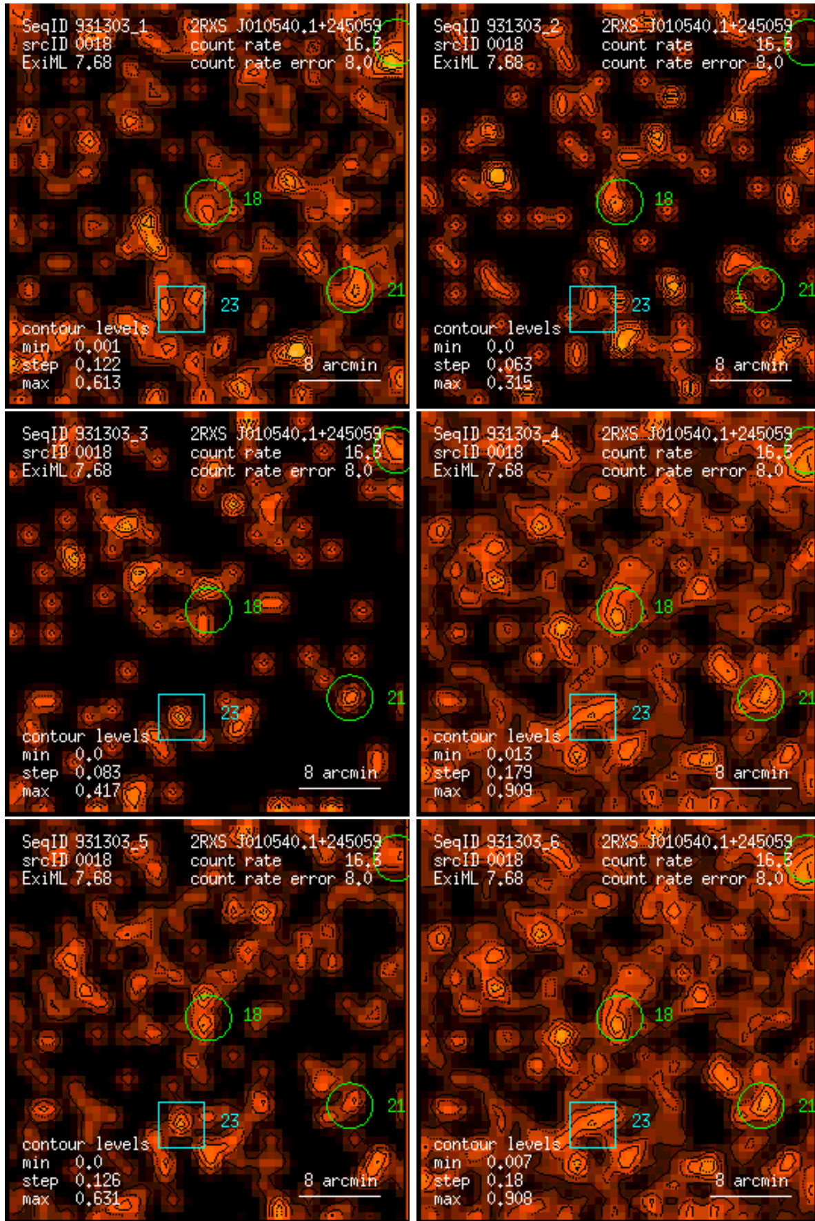
Figure 18: RASS 931303: detection 0018: band rate images, Gaussian filter: (1) PSPC channels 11 – 41, (2) 52 – 90, (3) 91 – 201, (4) 11 – 235, (5) 52 – 201, (6) 11 – 201. Broad band rates in counts/ks. Band rate contour levels in counts/ks/arcmin 2 .
