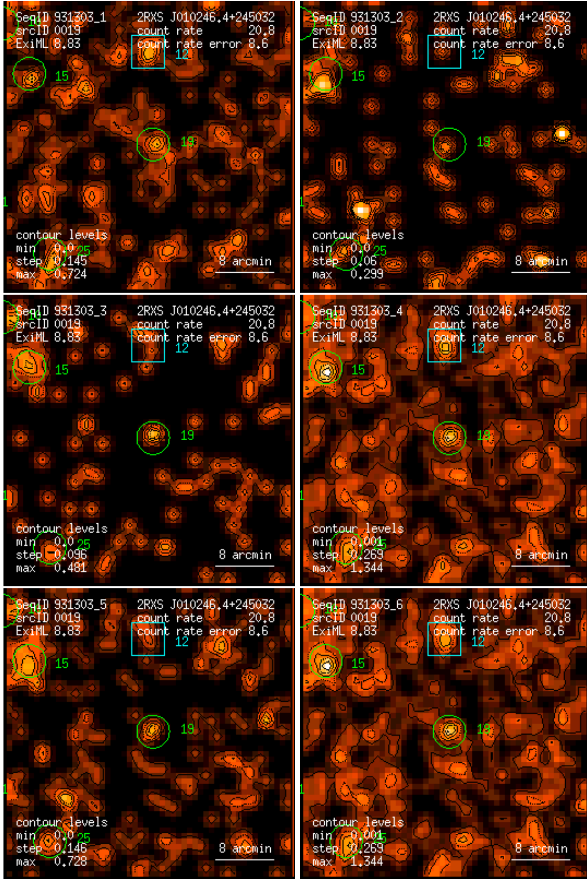
Figure 19: RASS 931303: detection 0019: band rate images, Gaussian filter: (1) PSPC channels 11 – 41, (2) 52 – 90, (3) 91 – 201, (4) 11 – 235, (5) 52 – 201, (6) 11 – 201. Broad band rates in counts/ks. Band rate contour levels in counts/ks/arcmin 2 .
