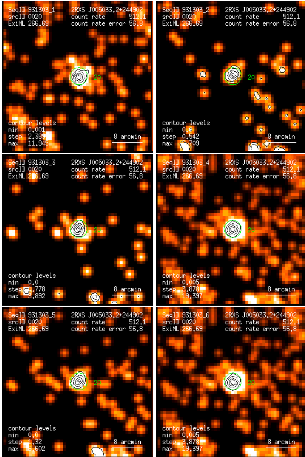
Figure 20: RASS 931303: detection 0020: band rate images, Gaussian filter: (1) PSPC channels 11 – 41, (2) 52 – 90, (3) 91 – 201, (4) 11 – 235, (5) 52 – 201, (6) 11 – 201. Broad band rates in counts/ks. Band rate contour levels in counts/ks/arcmin 2 .
