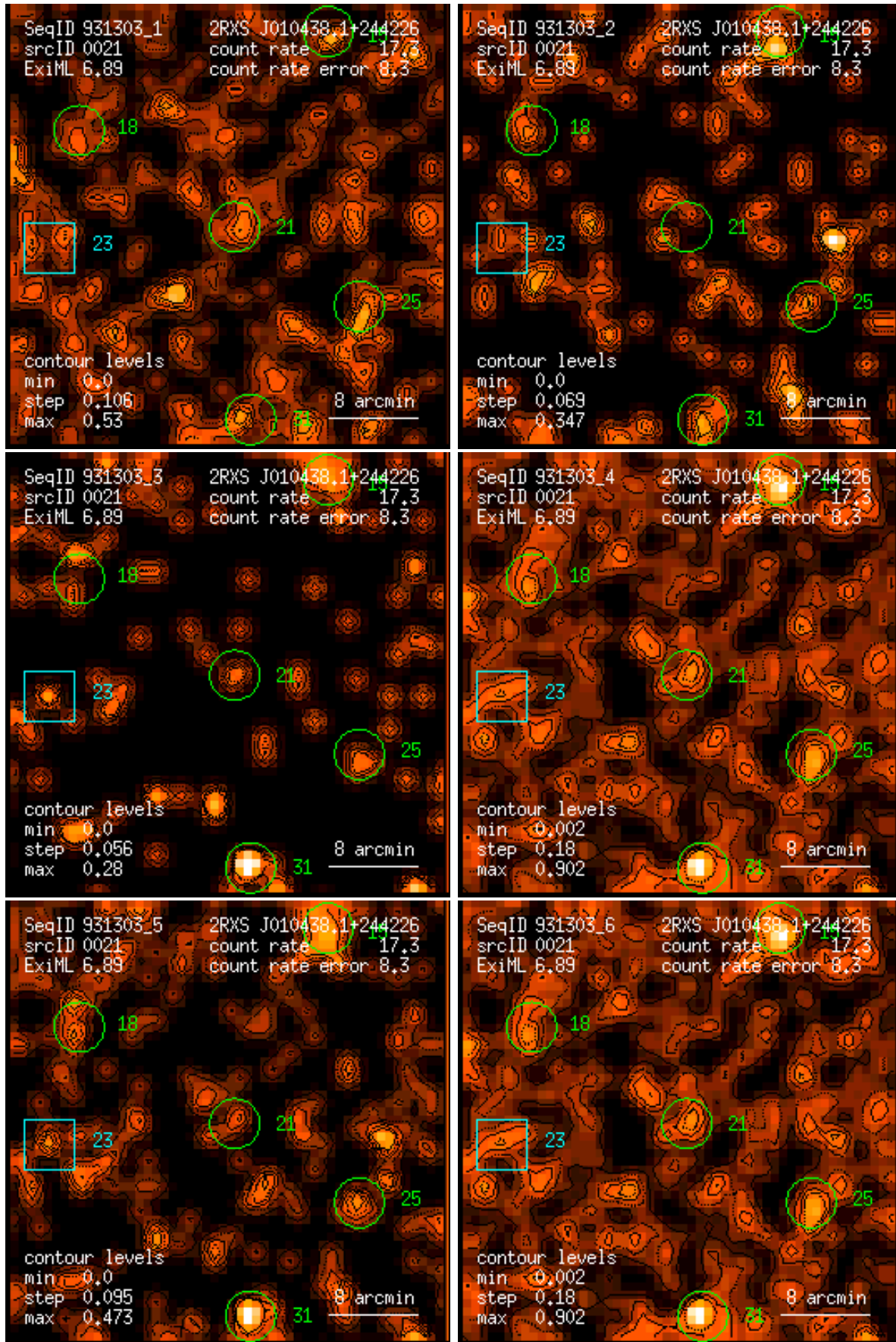
Figure 21: RASS 931303: detection 0021: band rate images, Gaussian filter: (1) PSPC channels 11 – 41, (2) 52 – 90, (3) 91 – 201, (4) 11 – 235, (5) 52 – 201, (6) 11 – 201. Broad band rates in counts/ks. Band rate contour levels in counts/ks/arcmin 2 .
