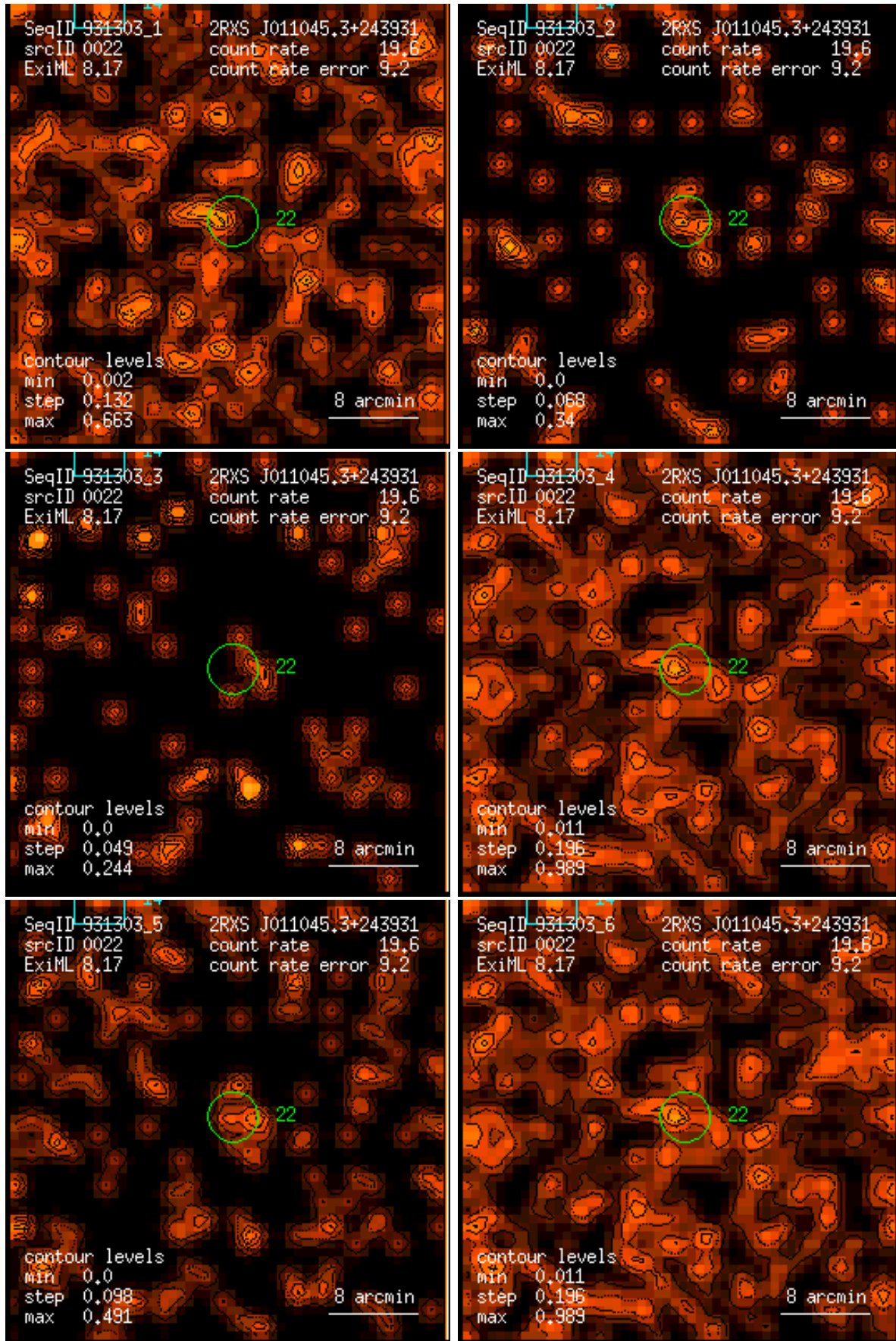
Figure 22: RASS 931303: detection 0022: band rate images, Gaussian filter: (1) PSPC channels 11 – 41, (2) 52 – 90, (3) 91 – 201, (4) 11 – 235, (5) 52 – 201, (6) 11 – 201. Broad band rates in counts/ks. Band rate contour levels in counts/ks/arcmin 2 .
