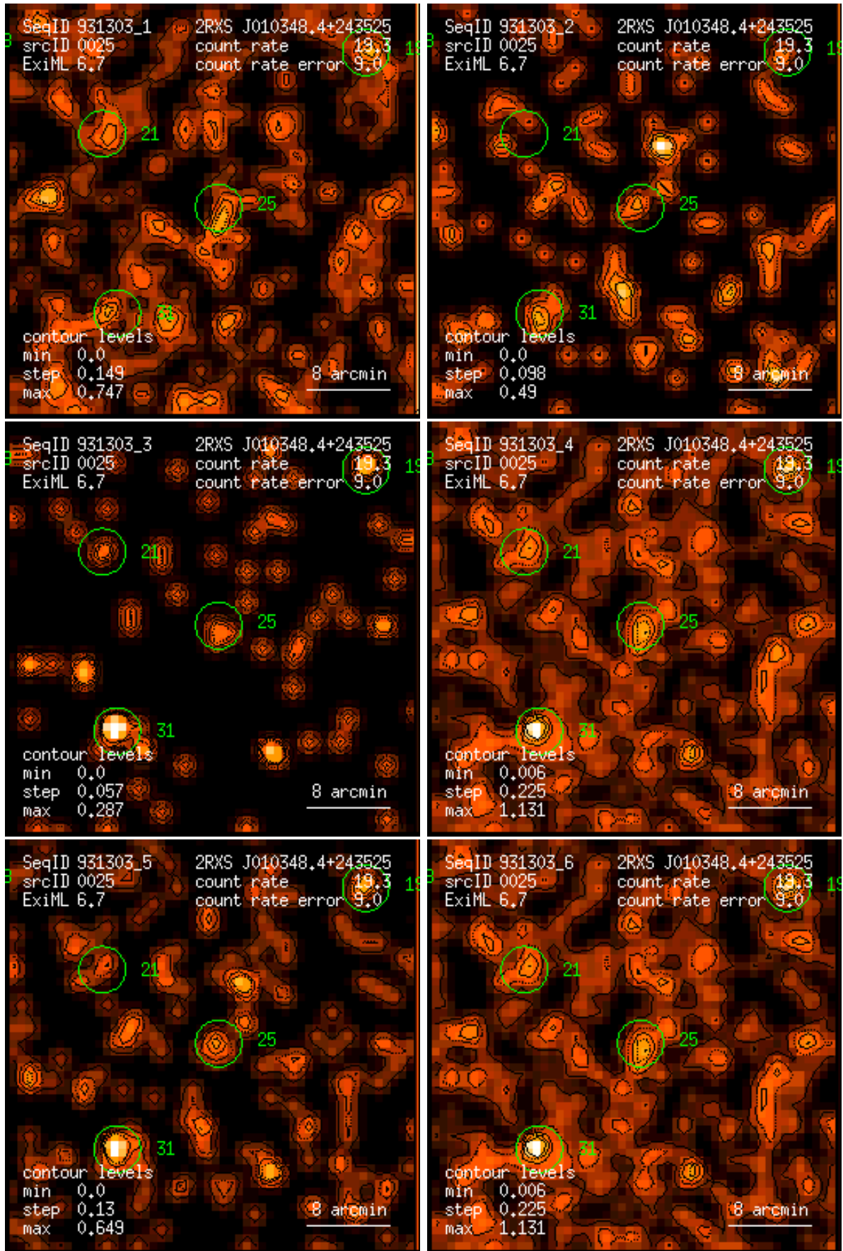
Figure 25: RASS 931303: detection 0025: band rate images, Gaussian filter: (1) PSPC channels 11 – 41, (2) 52 – 90, (3) 91 – 201, (4) 11 – 235, (5) 52 – 201, (6) 11 – 201. Broad band rates in counts/ks. Band rate contour levels in counts/ks/arcmin 2 .
