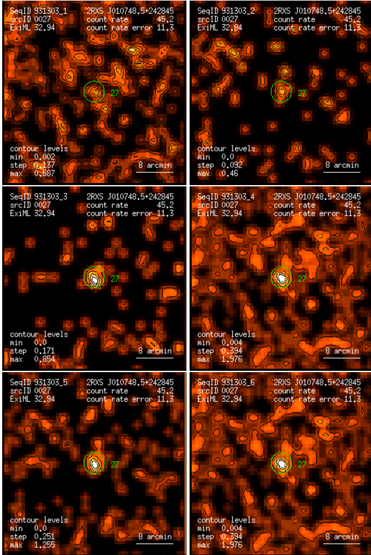
Figure 27: RASS 931303: detection 0027: band rate images, Gaussian filter: (1) PSPC channels 11 – 41, (2) 52 – 90, (3) 91 – 201, (4) 11 – 235, (5) 52 – 201, (6) 11 – 201. Broad band rates in counts/ks. Band rate contour levels in counts/ks/arcmin 2 .
