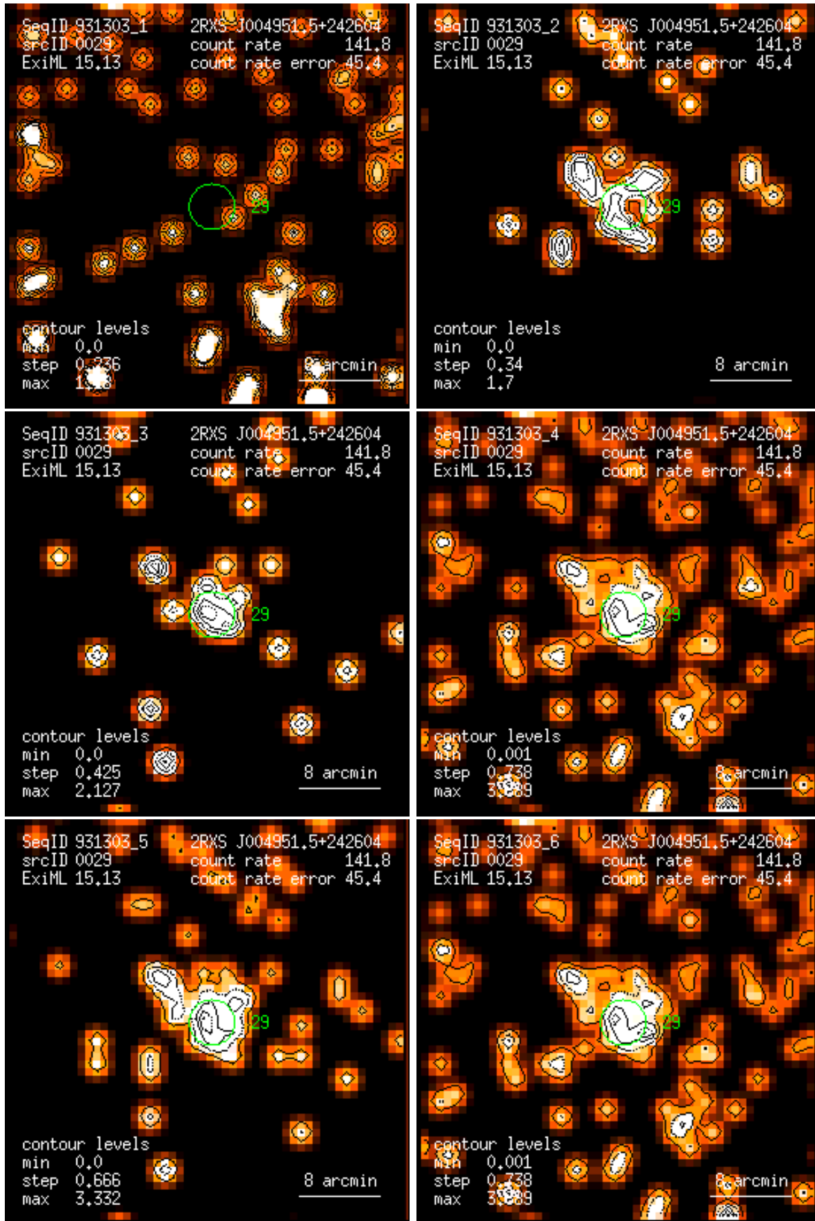
Figure 29: RASS 931303: detection 0029: band rate images, Gaussian filter: (1) PSPC channels 11 – 41, (2) 52 – 90, (3) 91 – 201, (4) 11 – 235, (5) 52 – 201, (6) 11 – 201. Broad band rates in counts/ks. Band rate contour levels in counts/ks/arcmin 2 .
