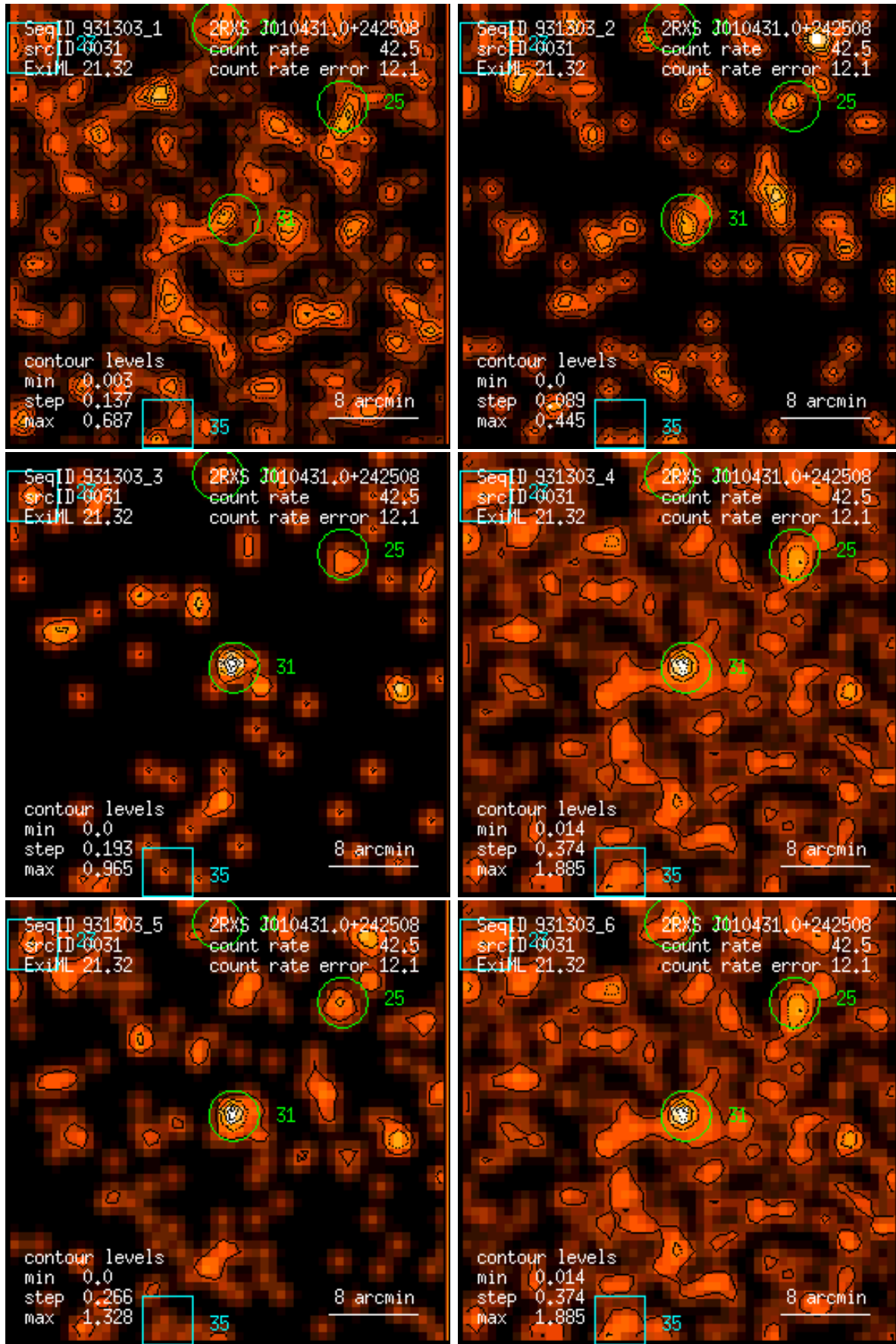
Figure 31: RASS 931303: detection 0031: band rate images, Gaussian filter: (1) PSPC channels 11 – 41, (2) 52 – 90, (3) 91 – 201, (4) 11 – 235, (5) 52 – 201, (6) 11 – 201. Broad band rates in counts/ks. Band rate contour levels in counts/ks/arcmin 2 .
