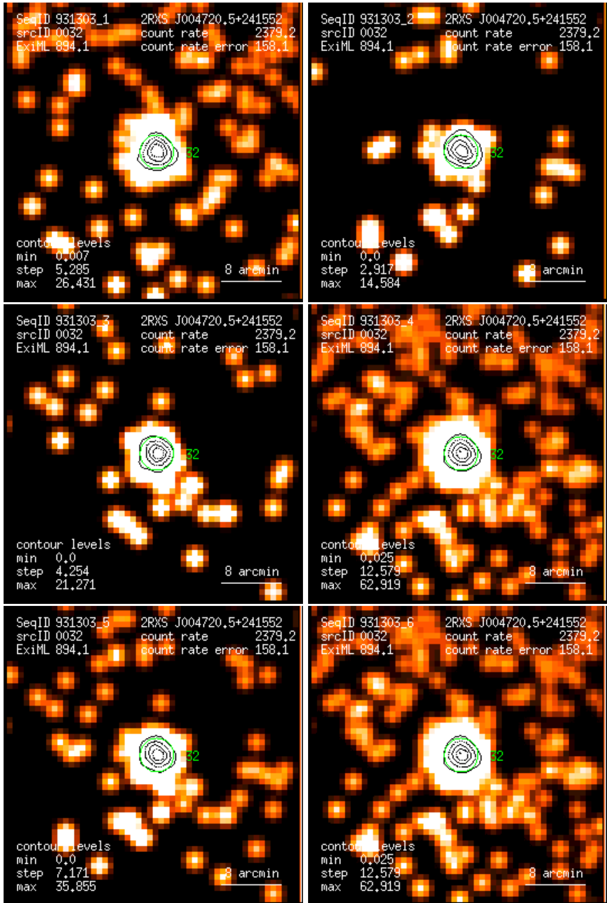
Figure 32: RASS 931303: detection 0032: band rate images, Gaussian filter: (1) PSPC channels 11 – 41, (2) 52 – 90, (3) 91 – 201, (4) 11 – 235, (5) 52 – 201, (6) 11 – 201. Broad band rates in counts/ks. Band rate contour levels in counts/ks/arcmin 2 .
