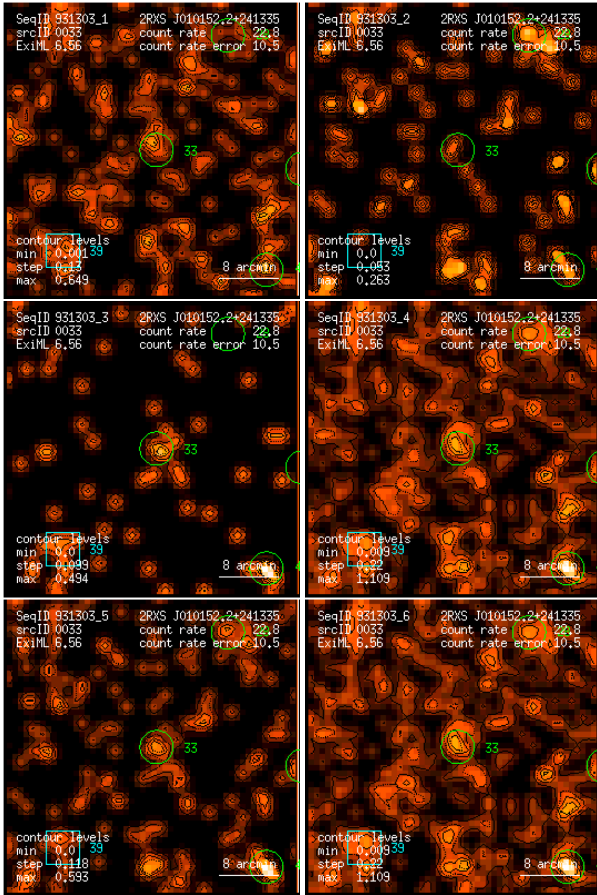
Figure 33: RASS 931303: detection 0033: band rate images, Gaussian filter: (1) PSPC channels 11 – 41, (2) 52 – 90, (3) 91 – 201, (4) 11 – 235, (5) 52 – 201, (6) 11 – 201. Broad band rates in counts/ks. Band rate contour levels in counts/ks/arcmin 2 .
