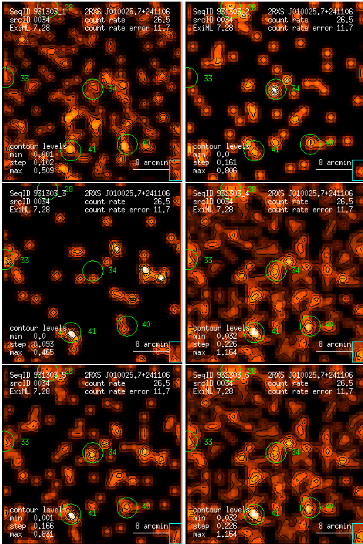
Figure 34: RASS 931303: detection 0034: band rate images, Gaussian filter: (1) PSPC channels 11 – 41, (2) 52 – 90, (3) 91 – 201, (4) 11 – 235, (5) 52 – 201, (6) 11 – 201. Broad band rates in counts/ks. Band rate contour levels in counts/ks/arcmin 2 .
