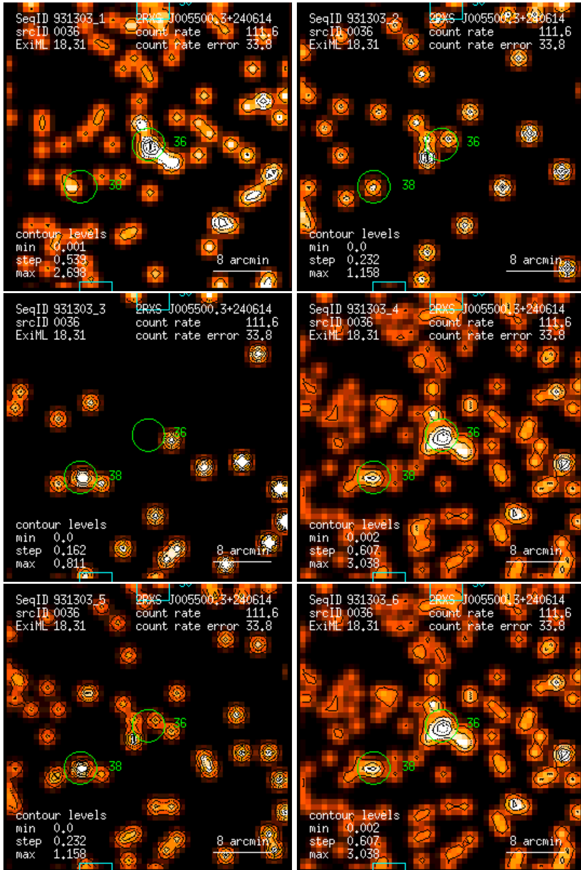
Figure 36: RASS 931303: detection 0036: band rate images, Gaussian filter: (1) PSPC channels 11 – 41, (2) 52 – 90, (3) 91 – 201, (4) 11 – 235, (5) 52 – 201, (6) 11 – 201. Broad band rates in counts/ks. Band rate contour levels in counts/ks/arcmin 2 .
