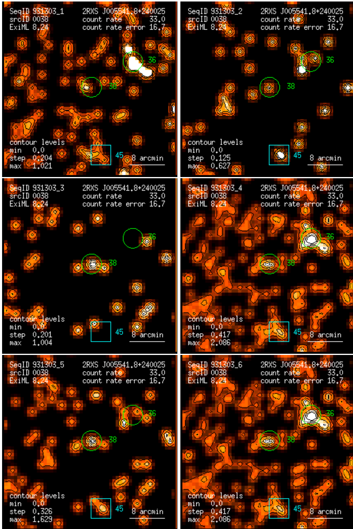
Figure 38: RASS 931303: detection 0038: band rate images, Gaussian filter: (1) PSPC channels 11 – 41, (2) 52 – 90, (3) 91 – 201, (4) 11 – 235, (5) 52 – 201, (6) 11 – 201. Broad band rates in counts/ks. Band rate contour levels in counts/ks/arcmin 2 .
