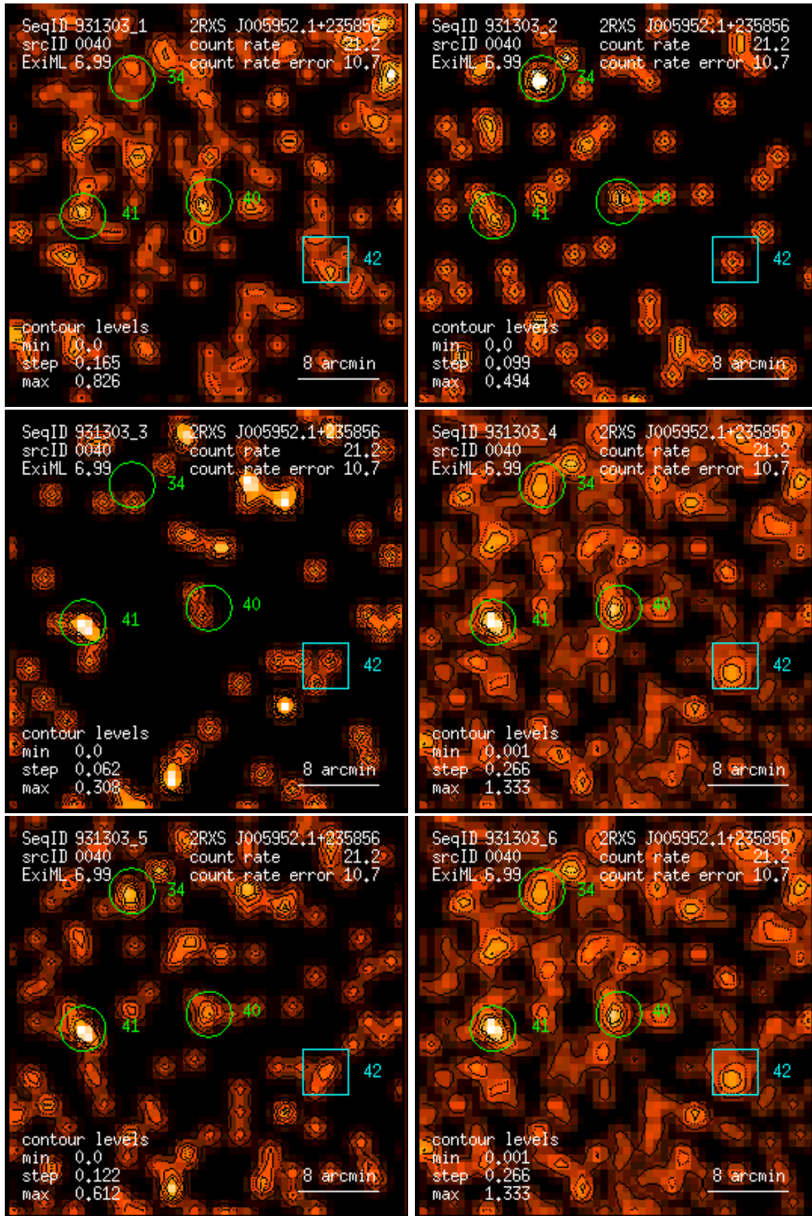
Figure 40: RASS 931303: detection 0040: band rate images, Gaussian filter: (1) PSPC channels 11 – 41, (2) 52 – 90, (3) 91 – 201, (4) 11 – 235, (5) 52 – 201, (6) 11 – 201. Broad band rates in counts/ks. Band rate contour levels in counts/ks/arcmin 2 .
