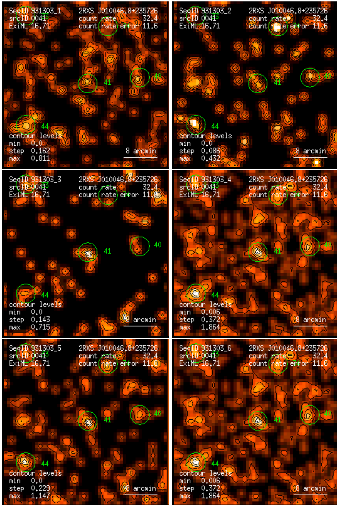
Figure 41: RASS 931303: detection 0041: band rate images, Gaussian filter: (1) PSPC channels 11 – 41, (2) 52 – 90, (3) 91 – 201, (4) 11 – 235, (5) 52 – 201, (6) 11 – 201. Broad band rates in counts/ks. Band rate contour levels in counts/ks/arcmin 2 .
