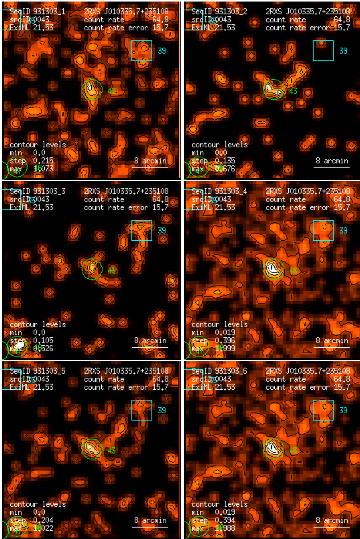
Figure 43: RASS 931303: detection 0043: band rate images, Gaussian filter: (1) PSPC channels 11 – 41, (2) 52 – 90, (3) 91 – 201, (4) 11 – 235, (5) 52 – 201, (6) 11 – 201. Broad band rates in counts/ks. Band rate contour levels in counts/ks/arcmin 2 .
