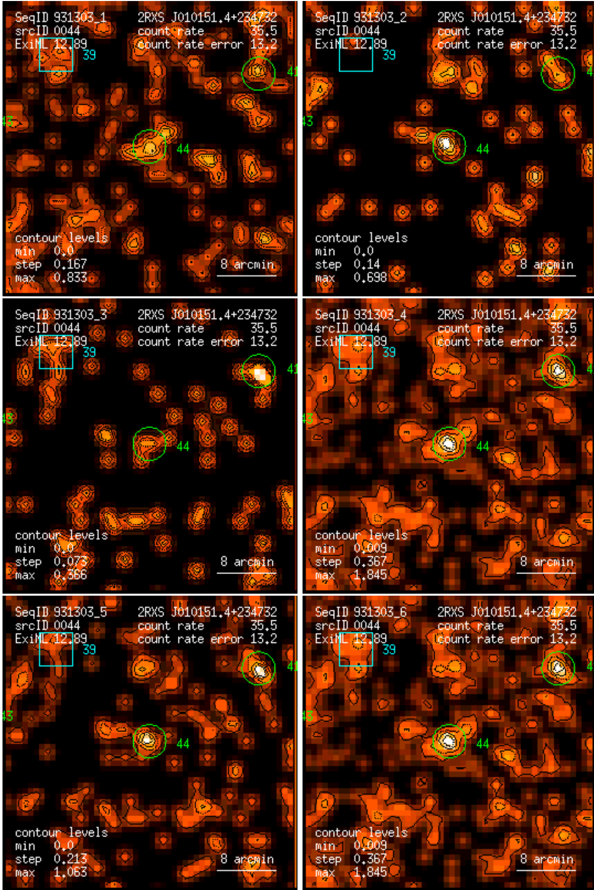
Figure 44: RASS 931303: detection 0044: band rate images, Gaussian filter: (1) PSPC channels 11 – 41, (2) 52 – 90, (3) 91 – 201, (4) 11 – 235, (5) 52 – 201, (6) 11 – 201. Broad band rates in counts/ks. Band rate contour levels in counts/ks/arcmin 2 .
