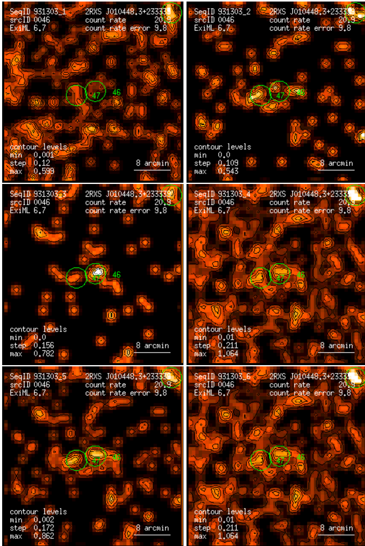
Figure 46: RASS 931303: detection 0046: band rate images, Gaussian filter: (1) PSPC channels 11 – 41, (2) 52 – 90, (3) 91 – 201, (4) 11 – 235, (5) 52 – 201, (6) 11 – 201. Broad band rates in counts/ks. Band rate contour levels in counts/ks/arcmin 2 .
