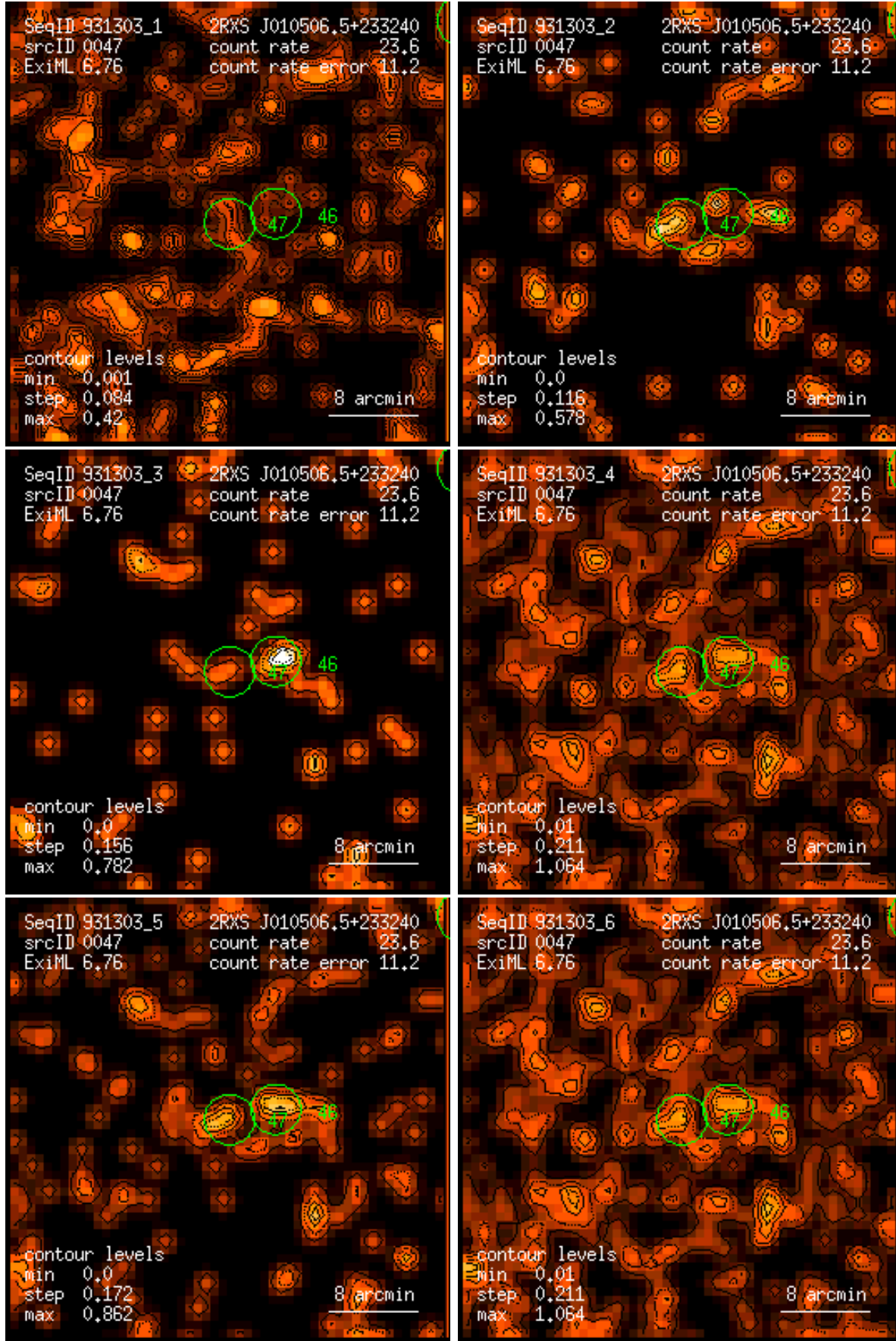
Figure 47: RASS 931303: detection 0047: band rate images, Gaussian filter: (1) PSPC channels 11 – 41, (2) 52 – 90, (3) 91 – 201, (4) 11 – 235, (5) 52 – 201, (6) 11 – 201. Broad band rates in counts/ks. Band rate contour levels in counts/ks/arcmin 2 .
