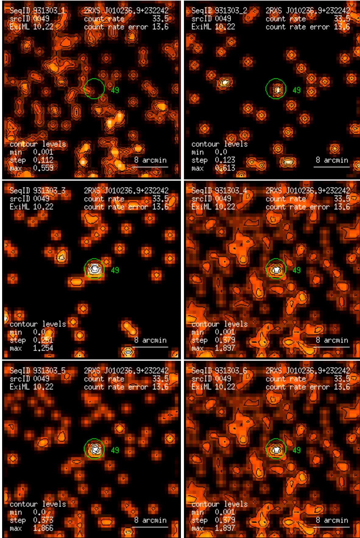
Figure 49: RASS 931303: detection 0049: band rate images, Gaussian filter: (1) PSPC channels 11 – 41, (2) 52 – 90, (3) 91 – 201, (4) 11 – 235, (5) 52 – 201, (6) 11 – 201. Broad band rates in counts/ks. Band rate contour levels in counts/ks/arcmin 2 .
