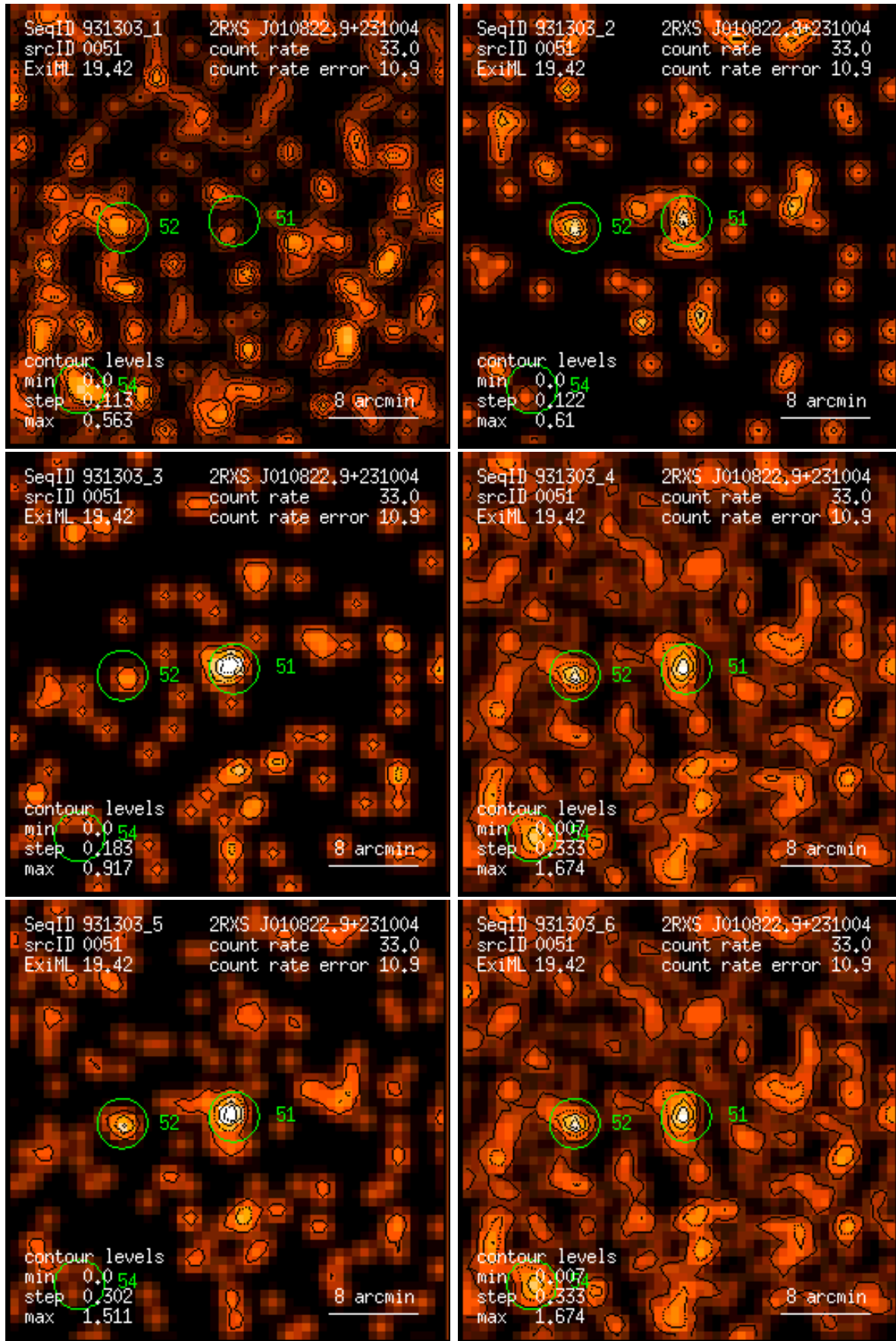
Figure 51: RASS 931303: detection 0051: band rate images, Gaussian filter: (1) PSPC channels 11 – 41, (2) 52 – 90, (3) 91 – 201, (4) 11 – 235, (5) 52 – 201, (6) 11 – 201. Broad band rates in counts/ks. Band rate contour levels in counts/ks/arcmin 2 .
