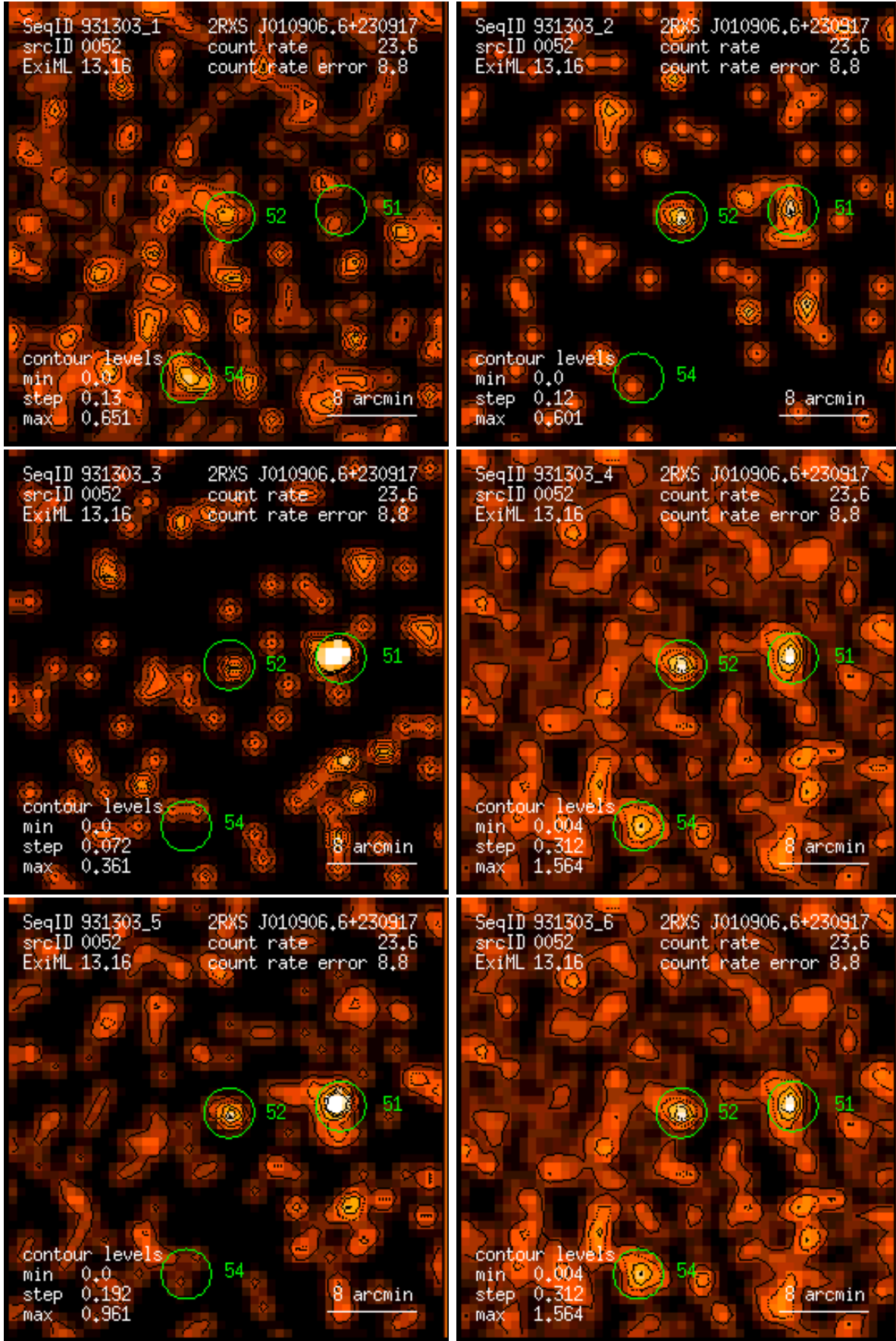
Figure 52: RASS 931303: detection 0052: band rate images, Gaussian filter: (1) PSPC channels 11 – 41, (2) 52 – 90, (3) 91 – 201, (4) 11 – 235, (5) 52 – 201, (6) 11 – 201. Broad band rates in counts/ks. Band rate contour levels in counts/ks/arcmin 2 .
