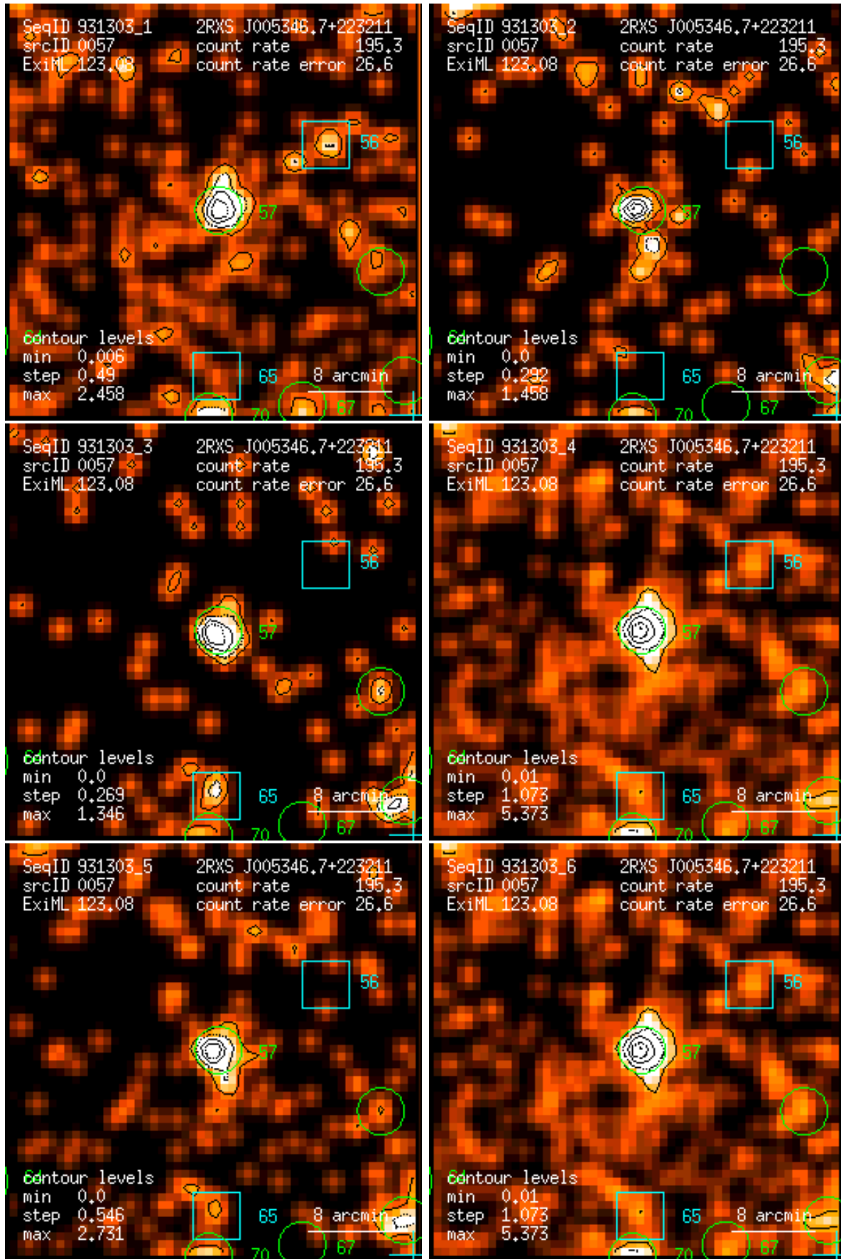
Figure 57: RASS 931303: detection 0057: band rate images, Gaussian filter: (1) PSPC channels 11 – 41, (2) 52 – 90, (3) 91 – 201, (4) 11 – 235, (5) 52 – 201, (6) 11 – 201. Broad band rates in counts/ks. Band rate contour levels in counts/ks/arcmin 2 .
