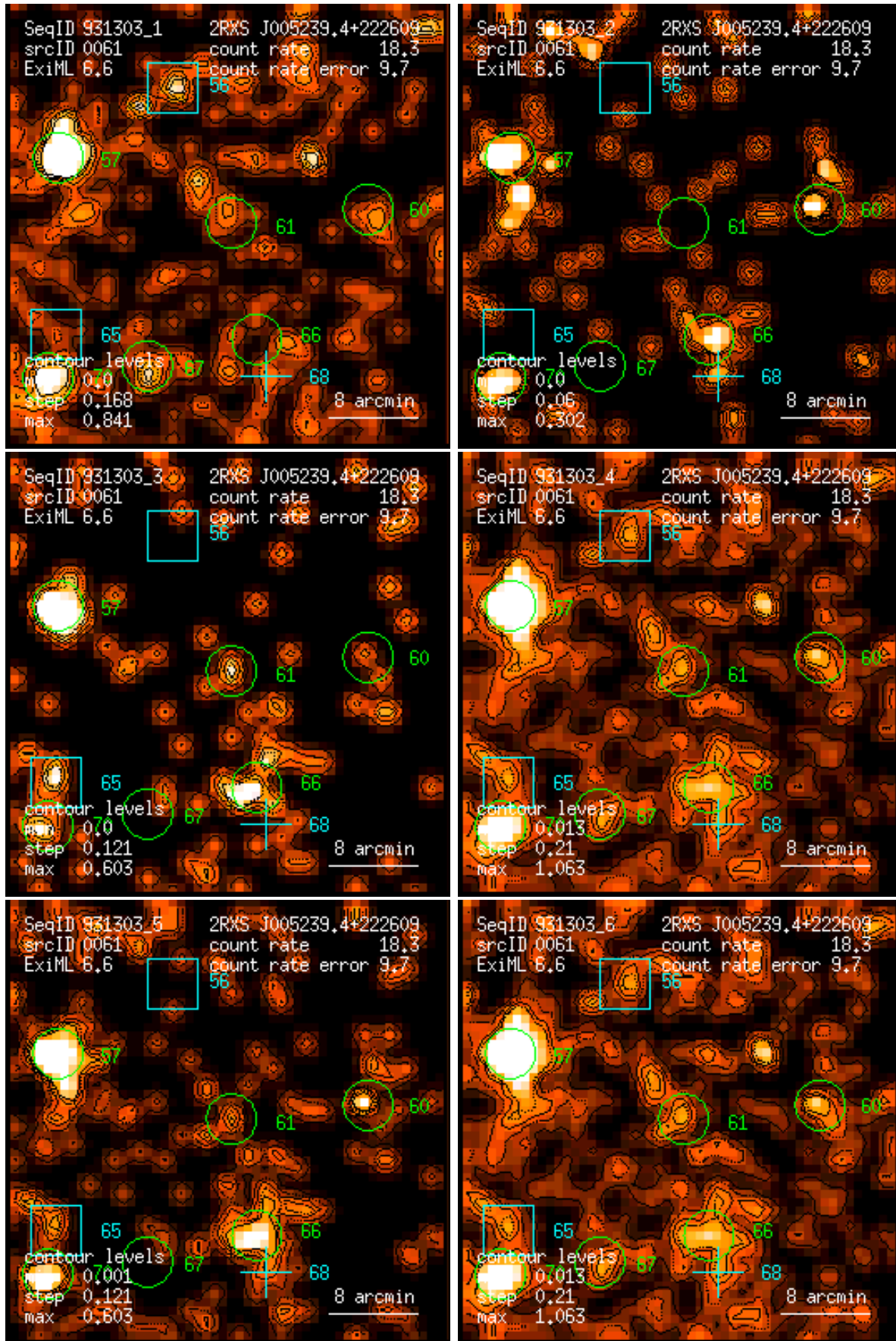
Figure 61: RASS 931303: detection 0061: band rate images, Gaussian filter: (1) PSPC channels 11 – 41, (2) 52 – 90, (3) 91 – 201, (4) 11 – 235, (5) 52 – 201, (6) 11 – 201. Broad band rates in counts/ks. Band rate contour levels in counts/ks/arcmin 2 .
