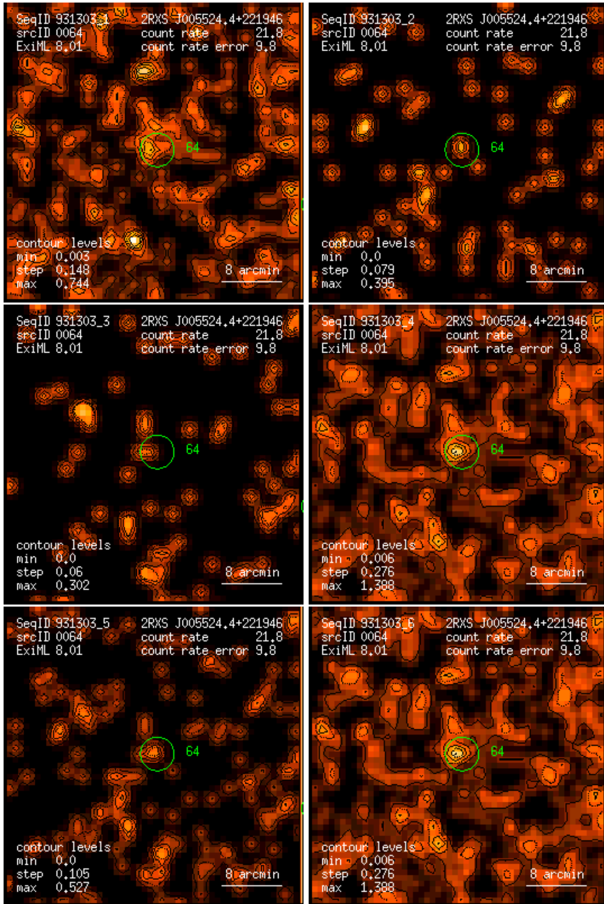
Figure 64: RASS 931303: detection 0064: band rate images, Gaussian filter: (1) PSPC channels 11 – 41, (2) 52 – 90, (3) 91 – 201, (4) 11 – 235, (5) 52 – 201, (6) 11 – 201. Broad band rates in counts/ks. Band rate contour levels in counts/ks/arcmin 2 .
