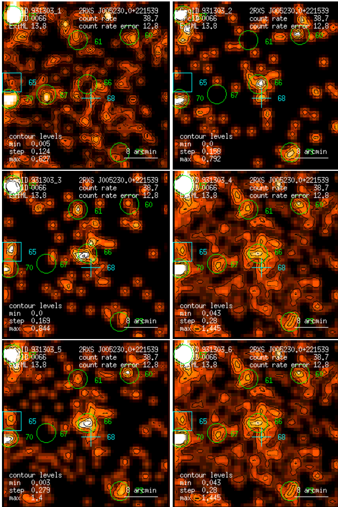
Figure 66: RASS 931303: detection 0066: band rate images, Gaussian filter: (1) PSPC channels 11 – 41, (2) 52 – 90, (3) 91 – 201, (4) 11 – 235, (5) 52 – 201, (6) 11 – 201. Broad band rates in counts/ks. Band rate contour levels in counts/ks/arcmin 2 .
