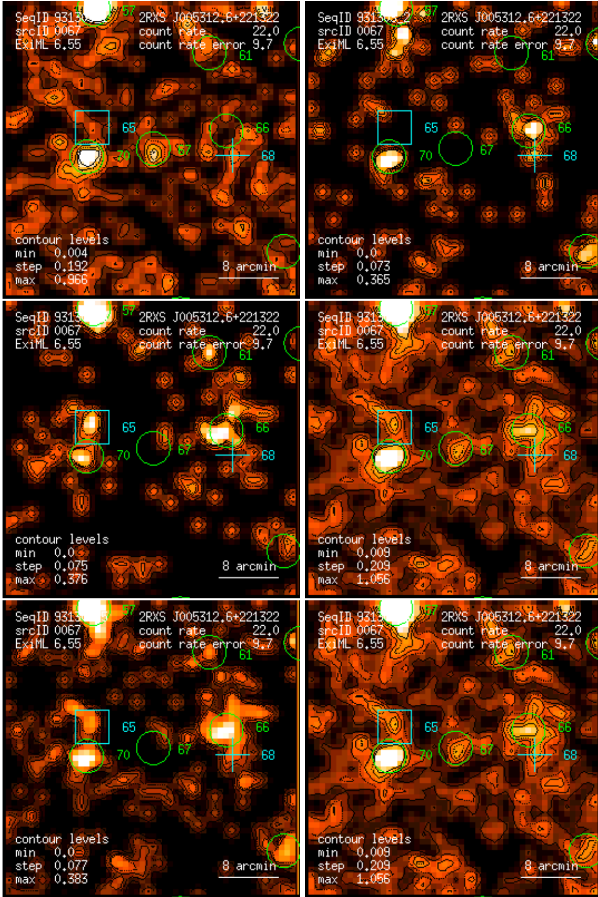
Figure 67: RASS 931303: detection 0067: band rate images, Gaussian filter: (1) PSPC channels 11 – 41, (2) 52 – 90, (3) 91 – 201, (4) 11 – 235, (5) 52 – 201, (6) 11 – 201. Broad band rates in counts/ks. Band rate contour levels in counts/ks/arcmin 2 .
