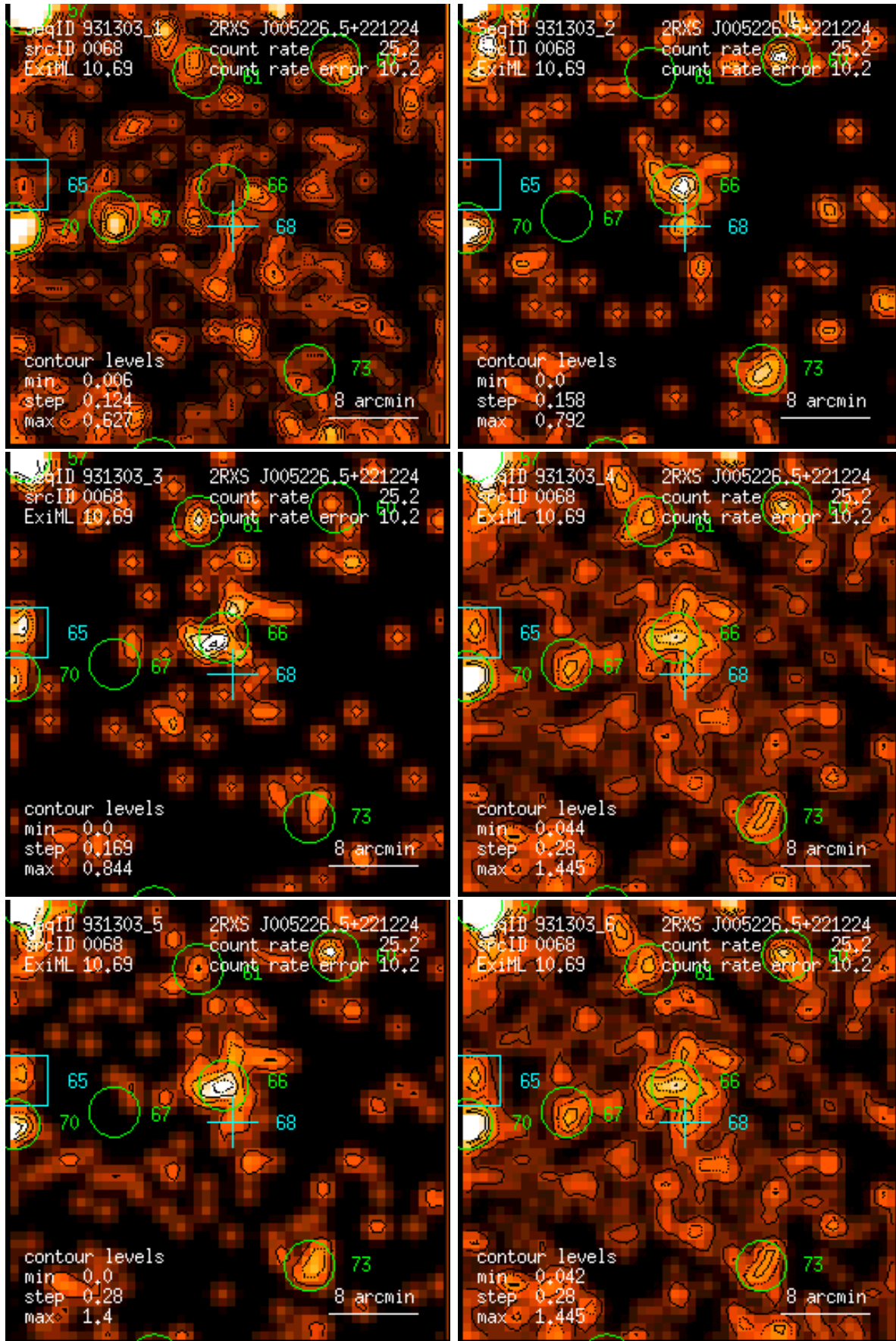
Figure 68: RASS 931303: detection 0068: band rate images, Gaussian filter: (1) PSPC channels 11 – 41, (2) 52 – 90, (3) 91 – 201, (4) 11 – 235, (5) 52 – 201, (6) 11 – 201. Broad band rates in counts/ks. Band rate contour levels in counts/ks/arcmin 2 .
