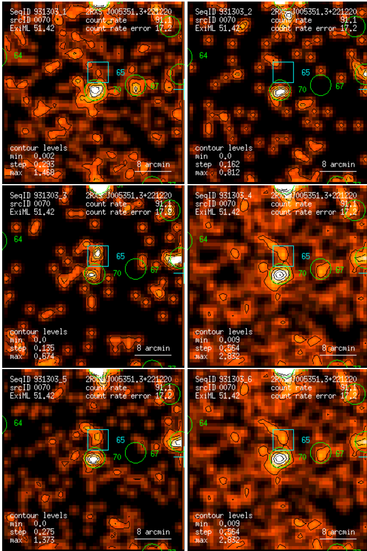
Figure 70: RASS 931303: detection 0070: band rate images, Gaussian filter: (1) PSPC channels 11 – 41, (2) 52 – 90, (3) 91 – 201, (4) 11 – 235, (5) 52 – 201, (6) 11 – 201. Broad band rates in counts/ks. Band rate contour levels in counts/ks/arcmin 2 .
